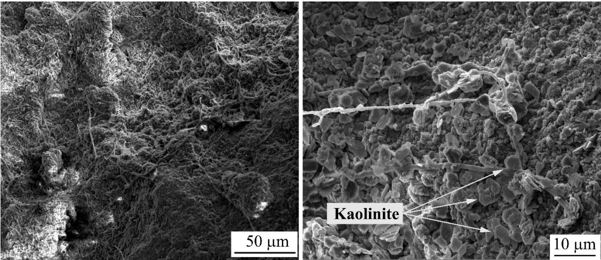
ESM_1pdf. Duman kaolinite deposit, footwall block, FE-SEM image of sample from mid-levels, retiform structures of the microbes on the kaolinite crystals.
