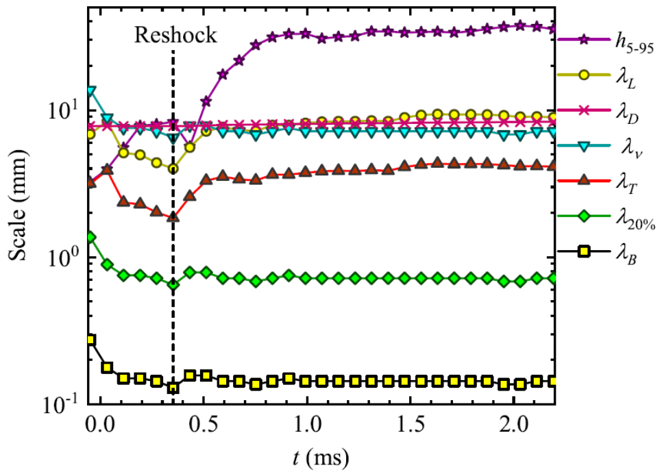
FIGURE. 12. Evolutions of turbulent length scales for case 3.
