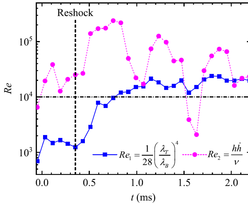
FIGURE. 9. Evolutions of Reynolds numbers for case 2.
