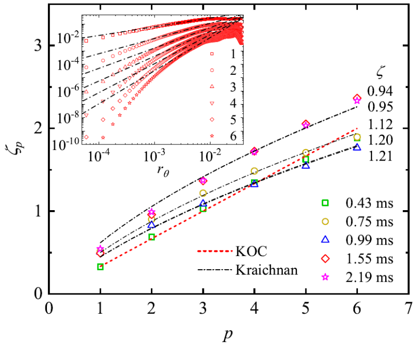
FIGURE. 14. Scaling law exponents of p -order structure functions for case 3.
