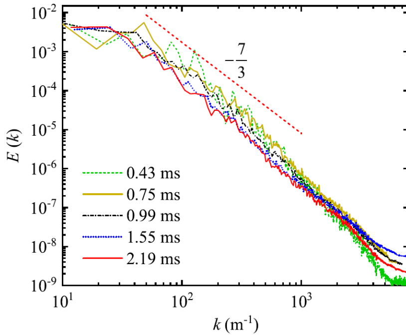
FIGURE. 8. The scalar energy spectra at times after reshock for case 3.
