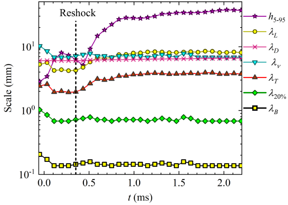
FIGURE. 11. Evolutions of turbulent length scales for case 2.
