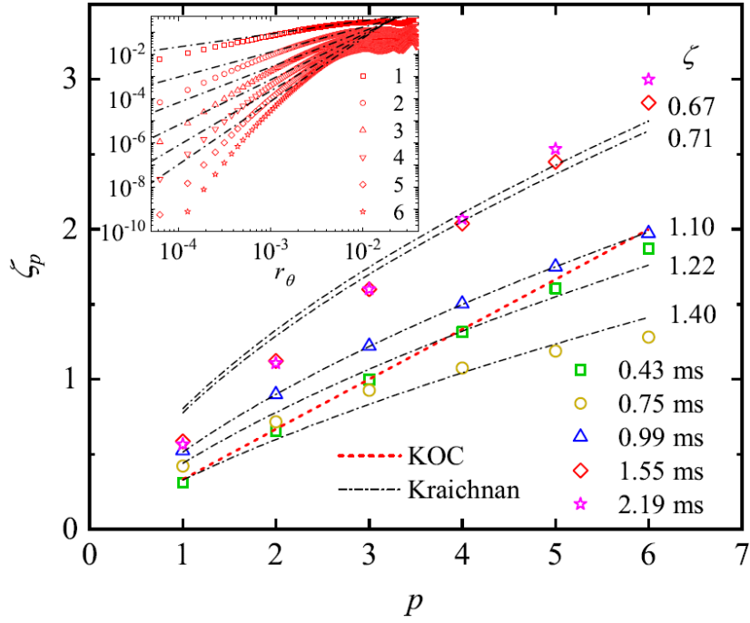
FIGURE. 13. Scaling law exponents of p -order structure functions for case 2.
