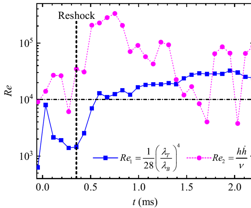
FIGURE. 10. Evolutions of Reynolds numbers for case 3.
