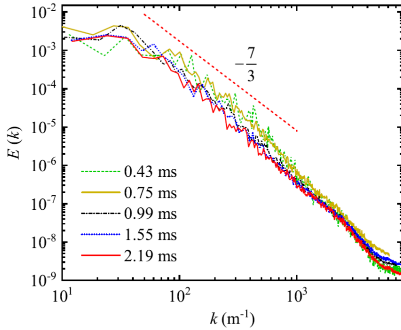
FIGURE. 7. The scalar energy spectra at times after reshock for case 2.
