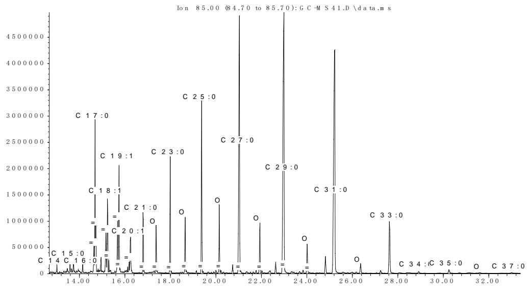
Fig.1 GC/MS of DKMD, YZF, QY, LHG, TS
