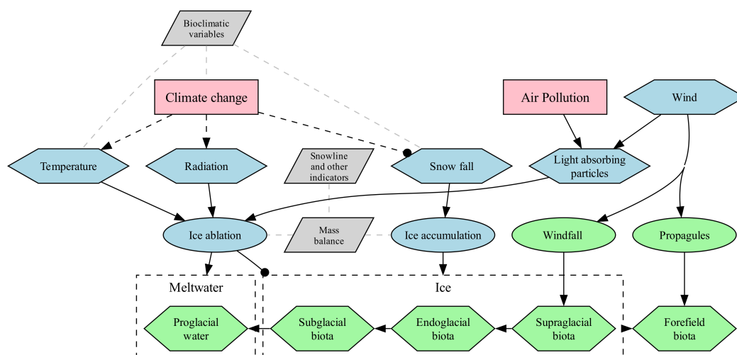
Figure 4: Conceptual Ecosystem Model for the Tropical glacier ecosystem of the Cordillera de Mérida
