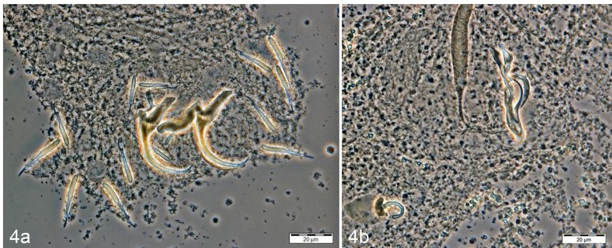
Fig. S4 Dactylogyrus rivalis n. sp. ex Squalius lepidus . Microphotograph of (a) the haptoral structures and (b) the male copulatory organ and vagina.
