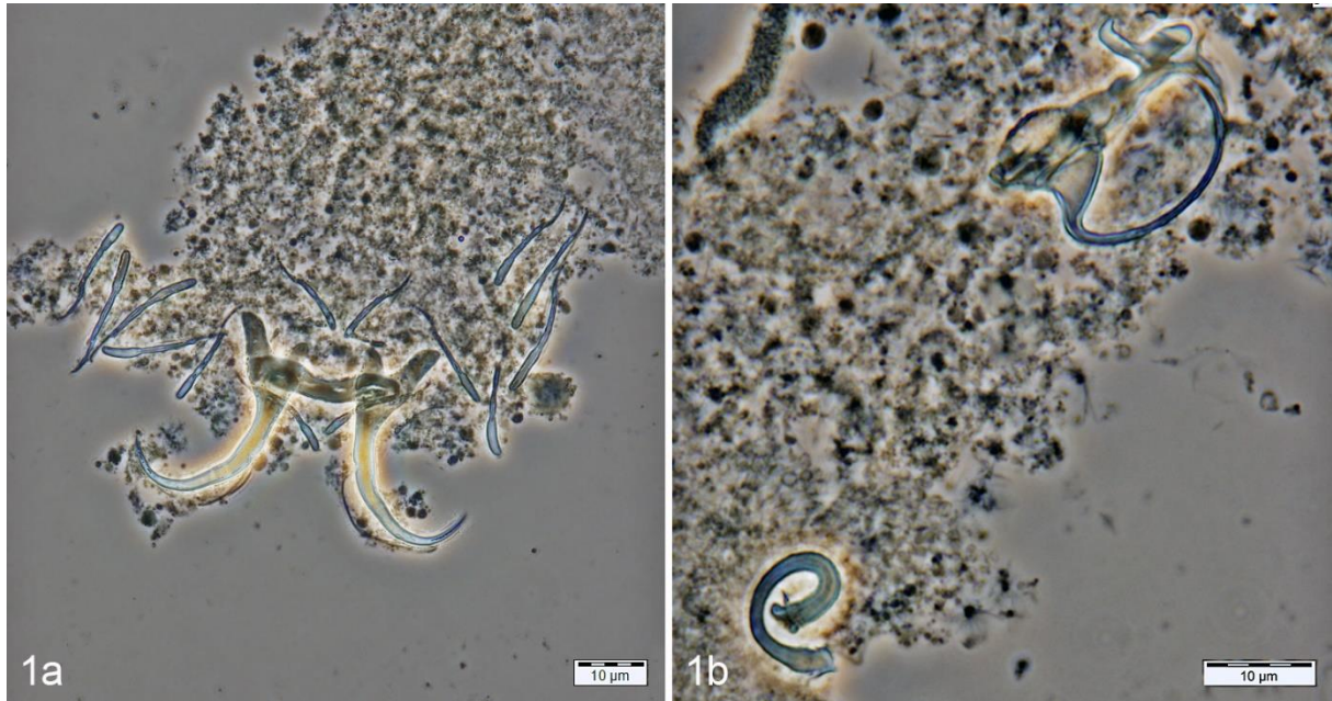
Fig. S1 Dactylogyrus anoigeus n. sp. ex Acanthobrama marmid . Microphotograph of (a) the haptor structures and (b) the male copulatory organ and vagina.
