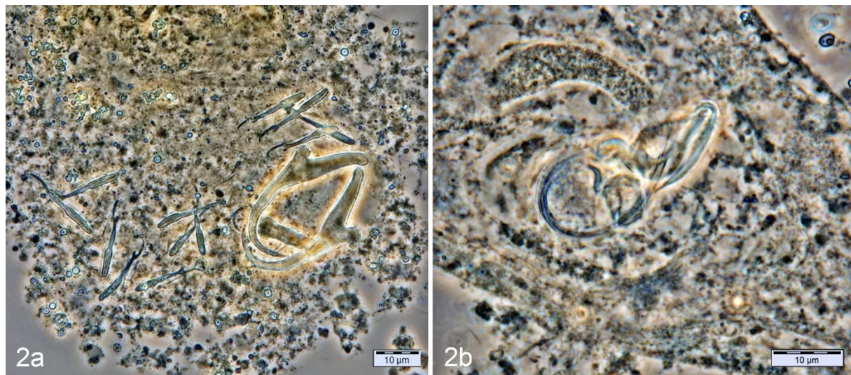
Fig. S2 Dactylogyrus medicus n. sp. ex Garra rufa . Microphotograph of (a) the haptor structures and (b) the male copulatory organ.
