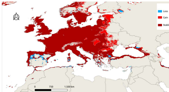
UKESM1-0-LL SSP3-7.0
