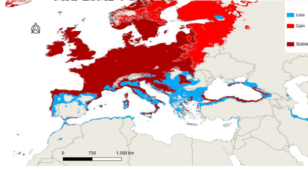
UKESM1-0-LL SSP5-8.5
