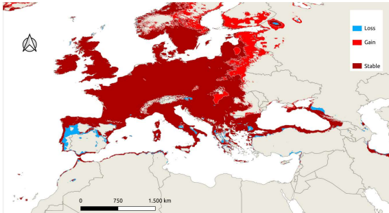
UKESM1-0-LL SSP3-7.0
