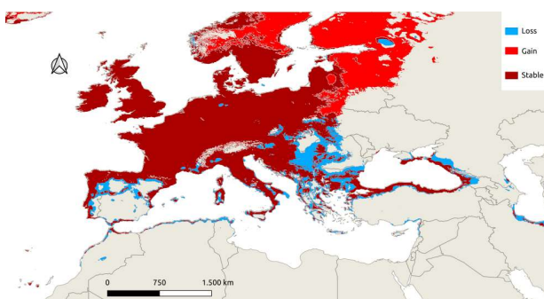
MRI-ESM2-0 SSP3-7.0
