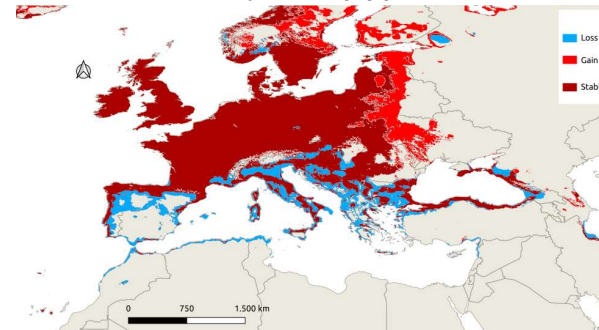
UKESM1-0-LL SSP5-8.5
