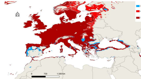
UKESM1-0-LL SSP5-8.5
