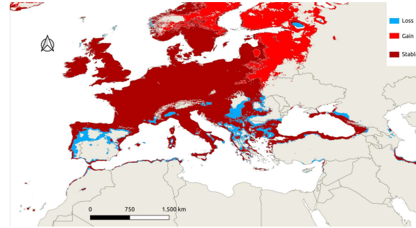
MRI-ESM2-0 SSP3-7.0
