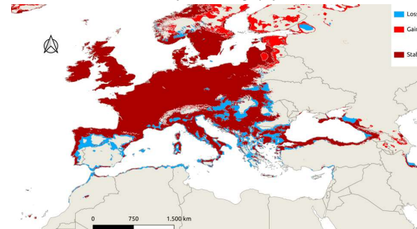
UKESM1-0-LL SSP3-7.0
