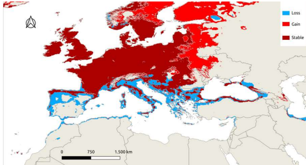
UKESM1-0-LL SSP3-7.0
