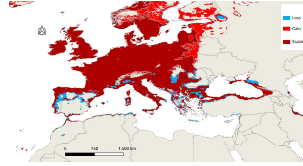
MRI-ESM2-0 SSP5-8.5
