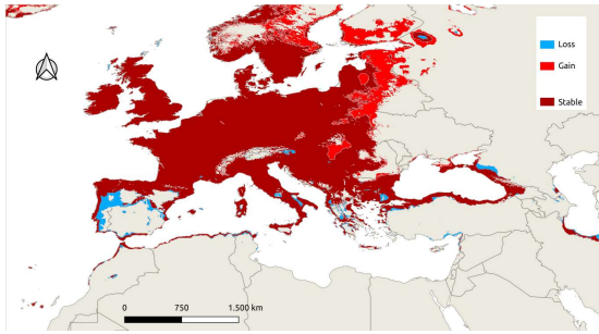
IPSL-CM6A-LR SSP3-7.0
