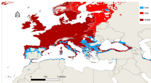
UKESM1-0-LL SSP3-7.0
