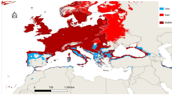
IPSL-CM6A-LR SSP3-7.0
