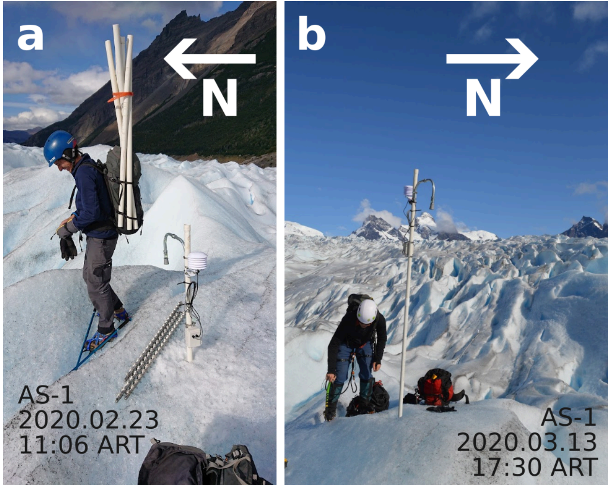
Supplementary Figure 1. Automated ablation stake AS-1 and ice-surface evolution during the measurement period. ART: Argentina Time, UTC-3. Pictured: (a) Guillermo Tamburini Beliveau, (b) Andy Wickert.
