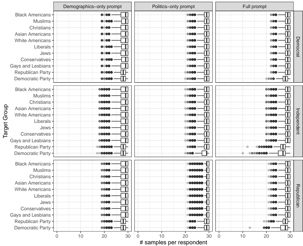
Figure 2: Number of synthetic responses by ANES respondent (x-axes) by target group (y-axes), detailed prompt type (columns), and synthetic party ID (rows).
