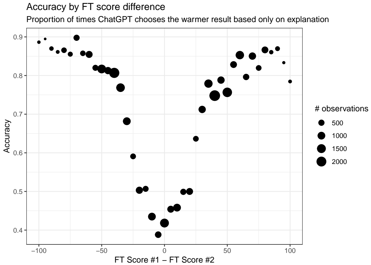
Figure 12: Relationship between difference in feeling thermometer scores (x-axis) and accuracy of ChatGPT 3.5-turbo adjudication between which explanation sounds warmer (y-axis).
