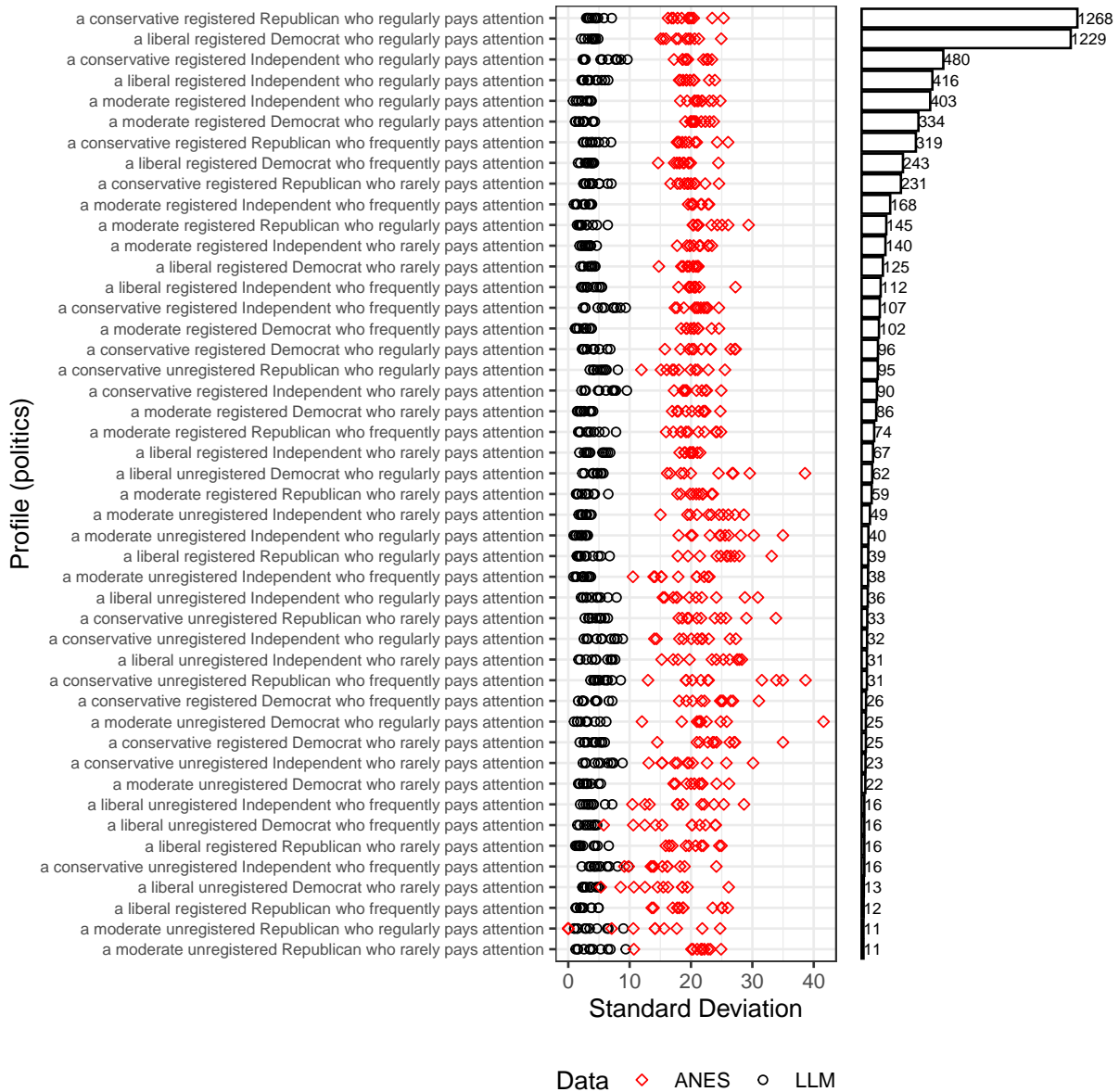
Figure 41: Standard deviation comparison between humans associated with a particular political profile (ideology by registration status by party ID by interest in news and politics, y-axis) indicated in red diamonds, compared to the standard deviation calculated among their synthetic counterparts indicated in black circles for the political profiles with more than 10 humans in them (total counts indicated by bars on right).
