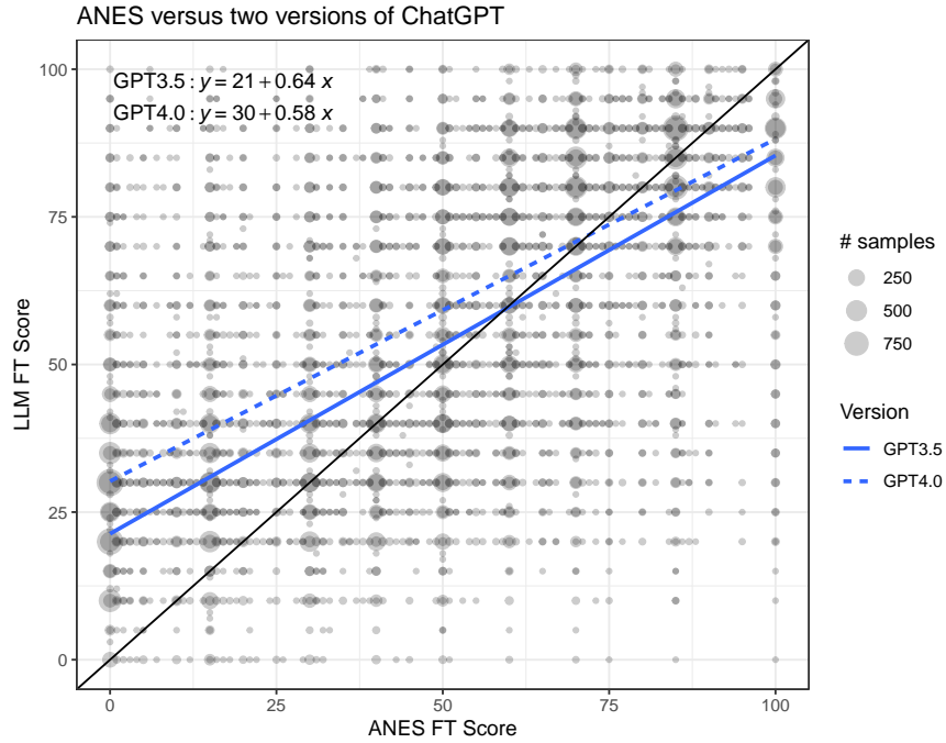
Figure 54: Scatterplot of human feelings toward various outgroups (x-axis) against their associated synthetic samples generated with ChatGPT 3.5-turbo (solid blue line) or ChatGPT 4.0 (dashed blue line). Points sized by the number of respondents associated with each pair of scores.
