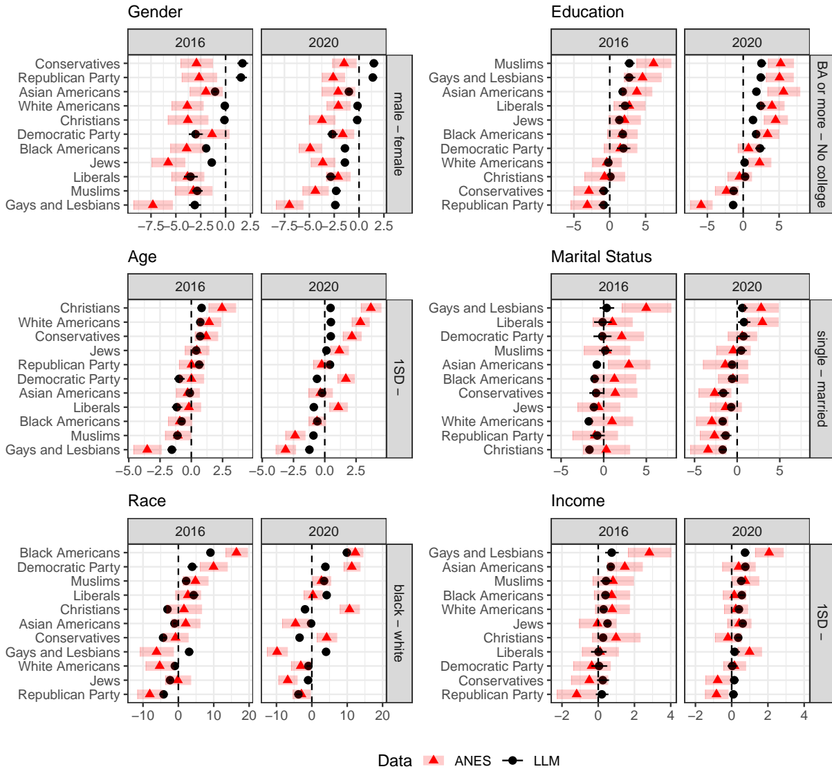
Figure 51: Regression coefficients estimated in either the ANES data (red triangles) or synthetic data generated by the detailed version of ChatGPT (black circles), along with two standard errors (thick red or thin black bars, respectively), by target group (y-axes), year (columns), and demographic covariate comparison (facets). Thus, for example, the top-left facet presents the regression coefficients capturing the difference between men and women in their feeling thermometer views towards different target groups in 2016 and 2020, highlighting that the synthetic data concludes that men are warmer toward conservatives in both years, while the ANES finds the opposite.
