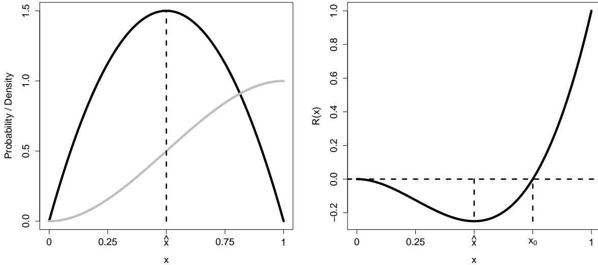
Figure C.1: Illustration of Lemma 1. The left panel shows the probability density function h (black line) and the cumulative distribution function H (gray line), where H = \mathcal{B}(2, 2) . The right panel shows the function R as defined in Definition 1.
