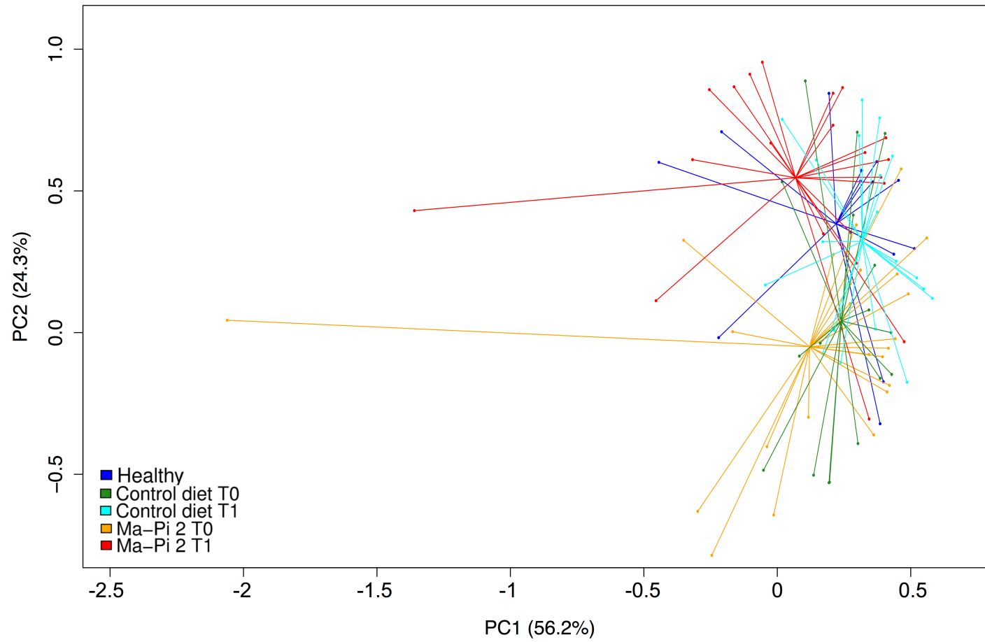
Supplemental Figure 5: PCoA analysis of the Hellinger distances between the imputed functional GM profiles of Healthy subjects (blue), CTR diet subjects at T0 (green) and T1 (cyan), Ma-Pi 2 subjects at T0 (orange) and T1 (red).
