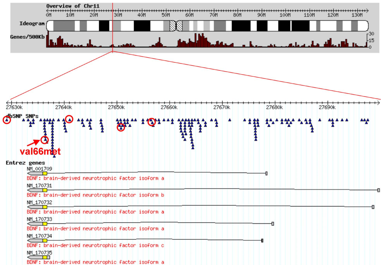
Fig. DS1 Schematic of BDNF located on the short arm of chromosome 11; six splice variants are depicted. The lone coding exon at the 3' end of the gene is at the left of the figure in yellow. Red circles designate the five single nucleotide polymorphisms (SNPs) genotyped for the present study. The SNP coding for the Val66Met amino acid substitution (rs6265) is indicated at the arrow.
