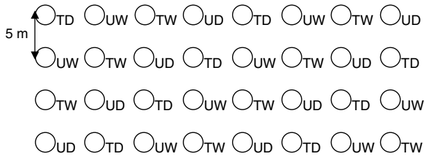
Fig. S4. Diagram of layout of traps baited with 'treated dry' (TD), 'treated wet' (TW), 'untreated dry' (UD) and 'untreated wet' (UW) dung for trial 3.
