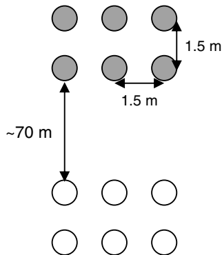
Fig. S2. Diagram showing the spatial location of pitfall traps baited with untreated dung (○) and treated dung (●) for trial 1.
