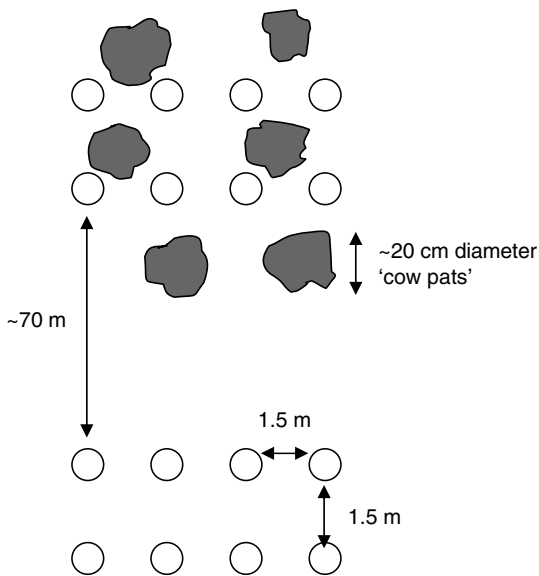
Fig. S5. Diagram of trap layout in trial 4 with pitfall traps baited with untreated dung and surrounded either by simulated cow pats or no cow pats.
