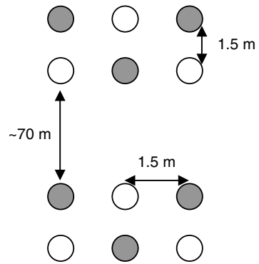
Fig. S3. Diagram showing the spatial location of pitfall traps baited with untreated dung (○) and treated dung (●) for trial 2.
