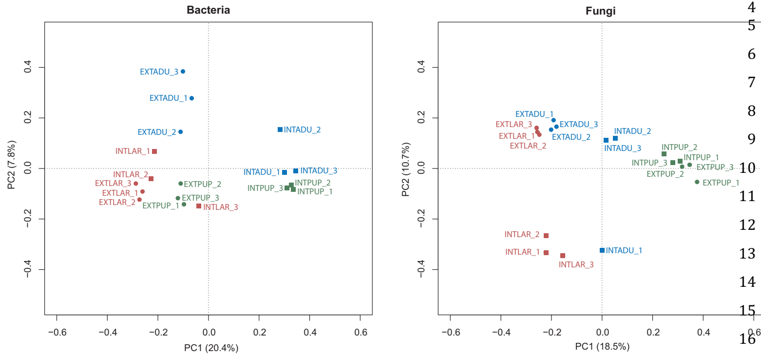
17 Figure S1. Principal component analysis of the different developmental stages and microenvironments of D. simplex for bacterial and fungal 18 microbiota. All generated OTU and equalized dataset has been used to generate the PCA. Numbers in parenthesis represent the percentage 19 explained by each axes. ECTO = ectomicrobiota, ENDO = endomicrobiota, ADU = adults, LAR = Larvae, PUP = Pupae.
