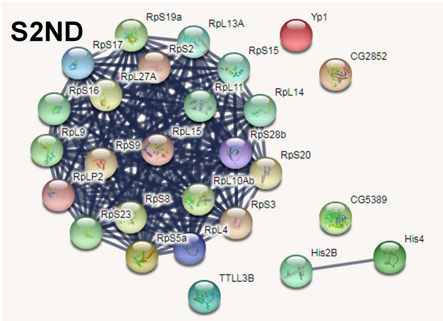
Supplementary Figure 3. Network of possible protein-protein interactions in non-diapausing (S2ND and S4ND), diapausing (S2D) and post-diapausing (S4PD) eggs of Mahanarva spectabilis . The interaction maps were generated by STRING 10.0 software. The codes in each node represent the proteins deposited in the STRING database.
