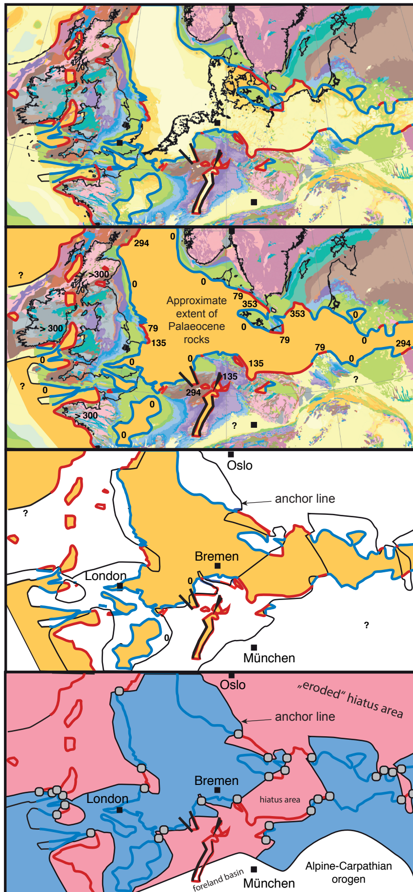
Figure SM 2. Same as Figure SM1 but for the base Palaeocene datum. Input map is the digital version of the IGME 5000 (Asch 2005).
