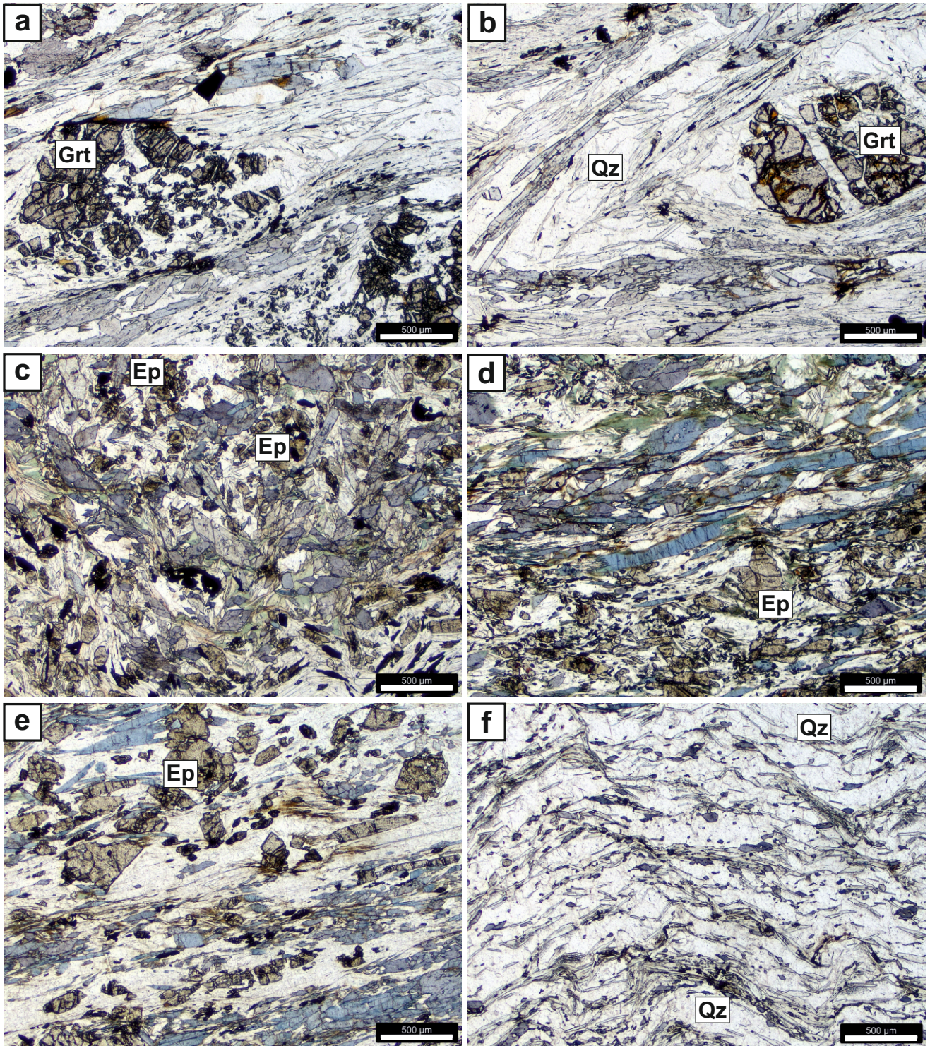
Figure S1. Photomicrographs of blueschist-facies samples from the Makrotantalón Unit that were used for Rb–Sr geochronology (plane-polarized light). (a) Sample 5776. (b) Sample 8104. (c) Sample 8111. (d) Sample 10AD37. (e) Sample 8192B. (f) Sample 1453, originally assigned to the Lower Unit (Bröcker & Franz, 2006). Ep = epidote; Grt = garnet; Qz = quartz. Scale bar is 500 µm across.
