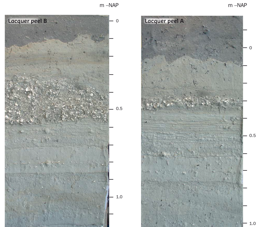
Fig. App. B8. Geoarchaeological survey in the pit Castricum - Zanderij. Location (CZ) is shown in Fig. 3.2.App. B
