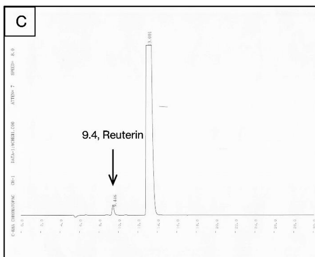
2 3 Supplementary figure 1. Chromatograms of glycerol (A), reuterin in the supernatant (B), and 4 reuterin after purification (C).
