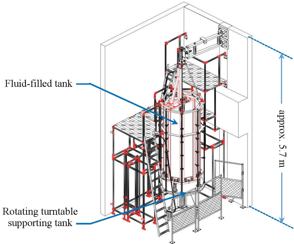
Figure S1. Technical drawing of the rotating-tank facility of the Fluid Dynamics Research Centre at the University of Warwick. The ejector box shown in figure 1 of the main article is located centrally at the bottom of the fluid-filled tank shown in figure S1.
