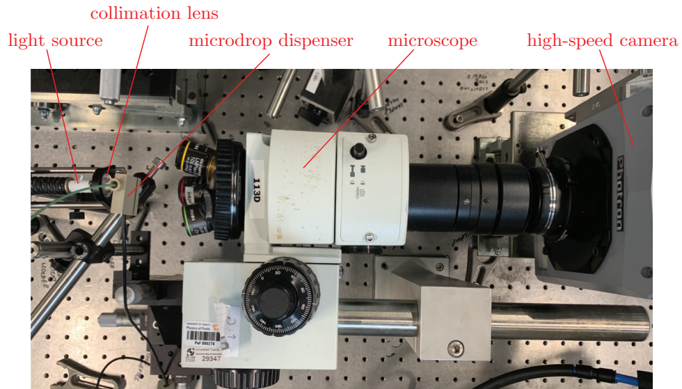
Figure S1: Top view photograph of the experimental setup
