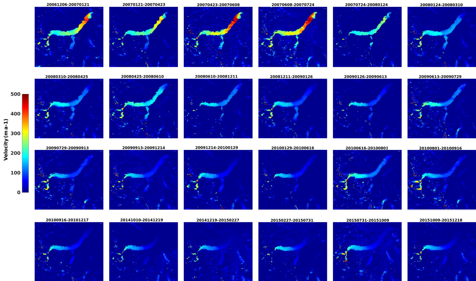
Figure S4. Surface velocity field of Gasherbrum Glacier from 2007 to 2015
