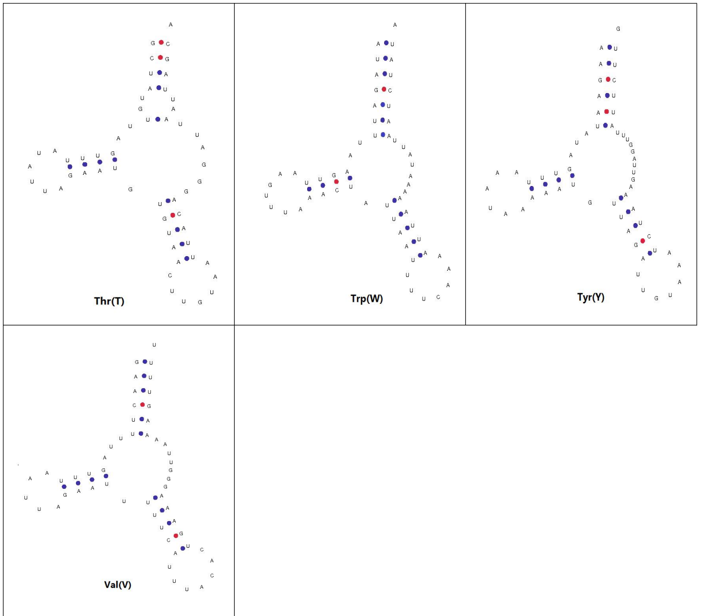
Fig. S1. Secondary structures predicted for the 22 tRNA genes in the mitochondrial genome of Cyathostomum pateratum
