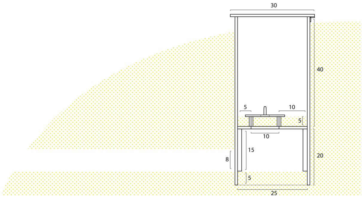
SUPPLEMENTARY FIG. 1 Design of a Whenua Hou diving petrel Pelecanoides whenuahouensis nest box, following Fischer et al. (2018a). Dimensions are in cm.
