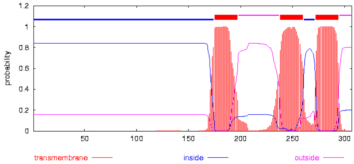
TMHMM posterior probabilities for Sequence
