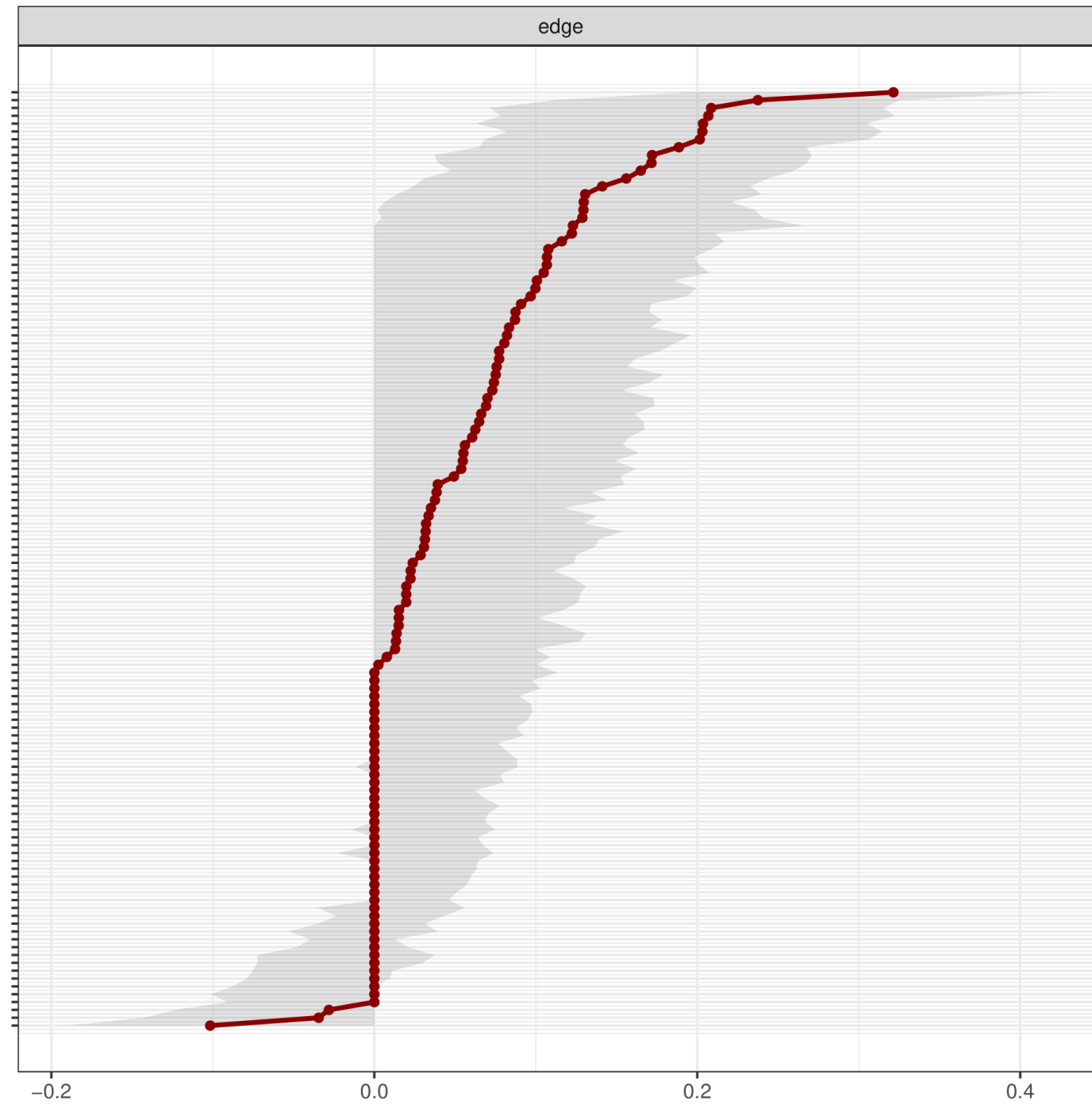
Fig. S3. Bootstrapped Confidence Intervals of edge-weights for the PCBD networks. Red lines represent edges, ordered by edge weight magnitude, and the gray areas represent their bootstrapped CIs.
