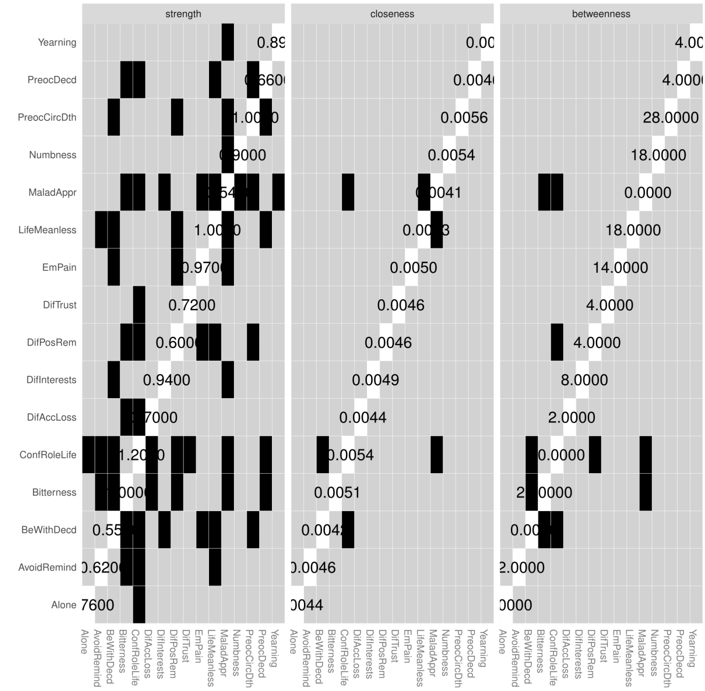
Fig. S4. Bootstrapped difference significance tests between PCBD node centrality indices. Black boxes represent nodes that do differ significantly from one-another. Numbers show the values of the node's Strength.
