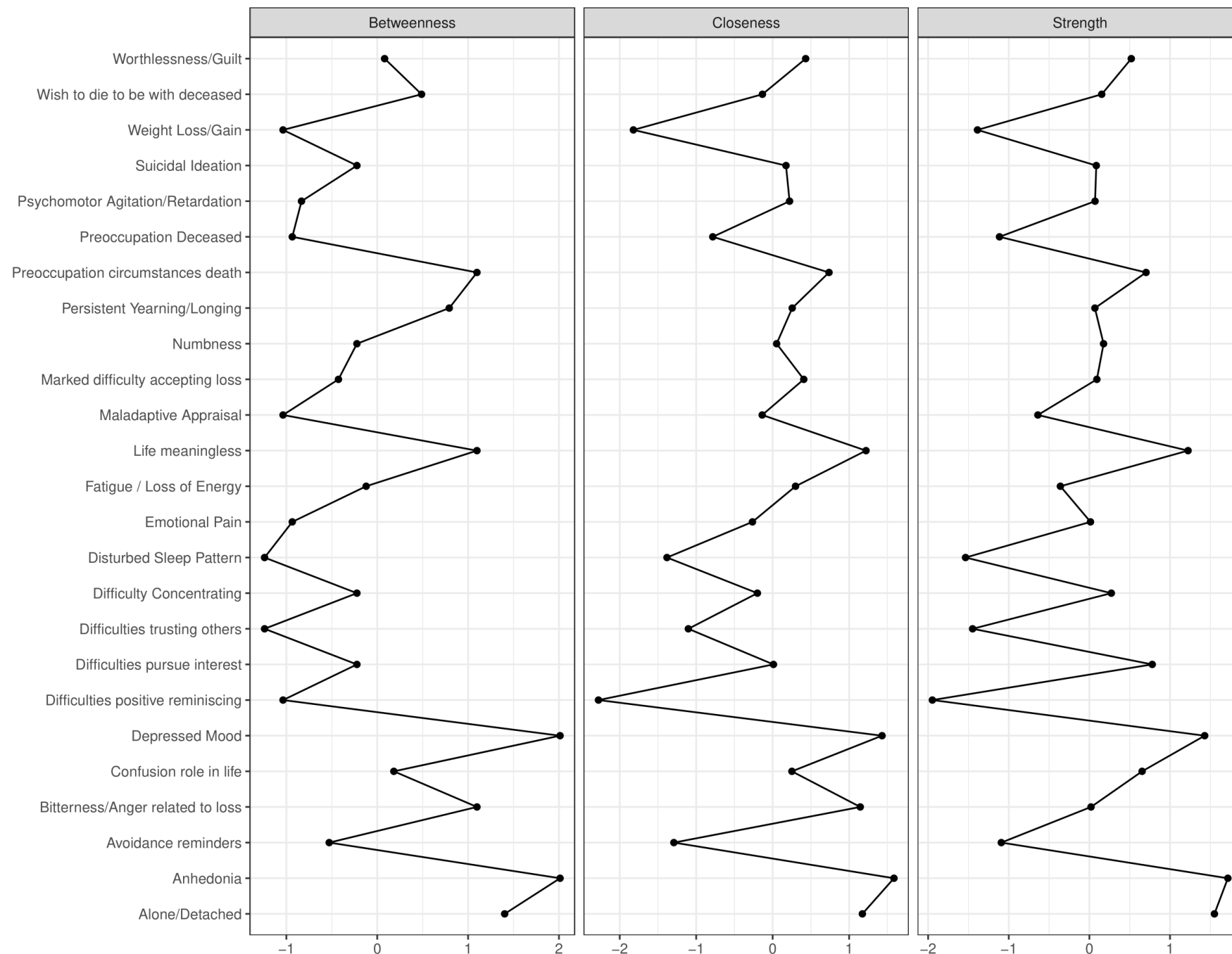
Fig. S6. Comparison of centrality indices for PCBD and MDD at 14 months post-loss.
