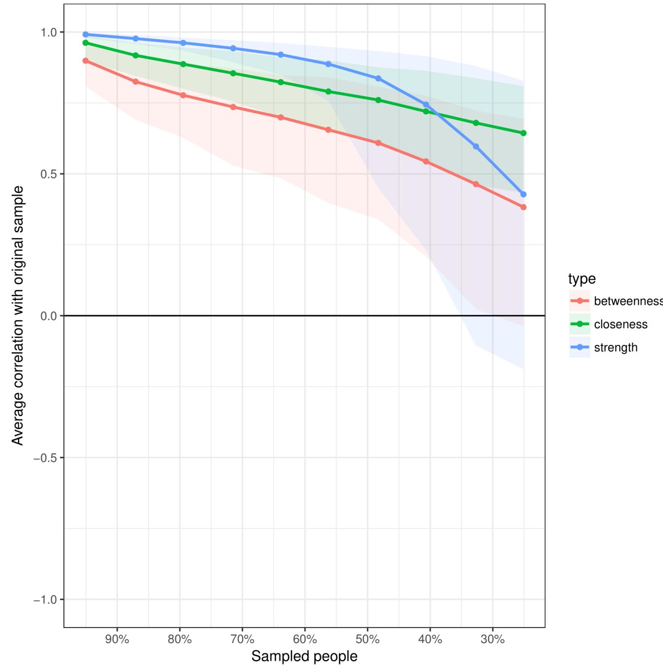
Fig. S12. PCBD/PTSD Networks average correlations between centrality indices from the original sample and from networks sampled with increasing percentages of dropped participants. Lines indicate the centrality scores means and areas indicate their 95% CIs. Centrality estimates can be considered stable when the correlation after dropping a substantial amount of participants remains high.
