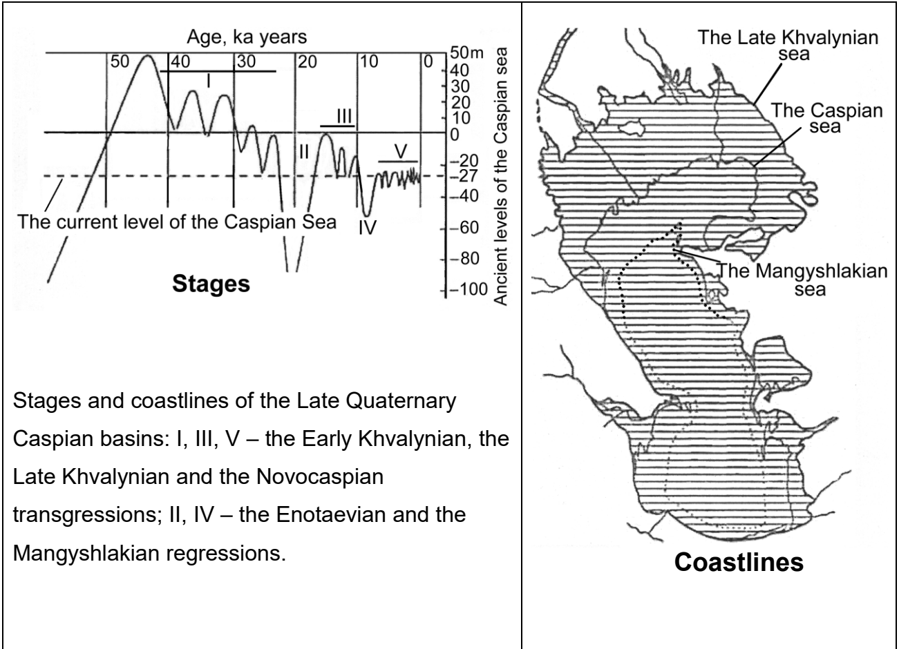
Supplementary Figure 1. Fluctuations of the Caspian Sea level during the Late Quaternary time.
