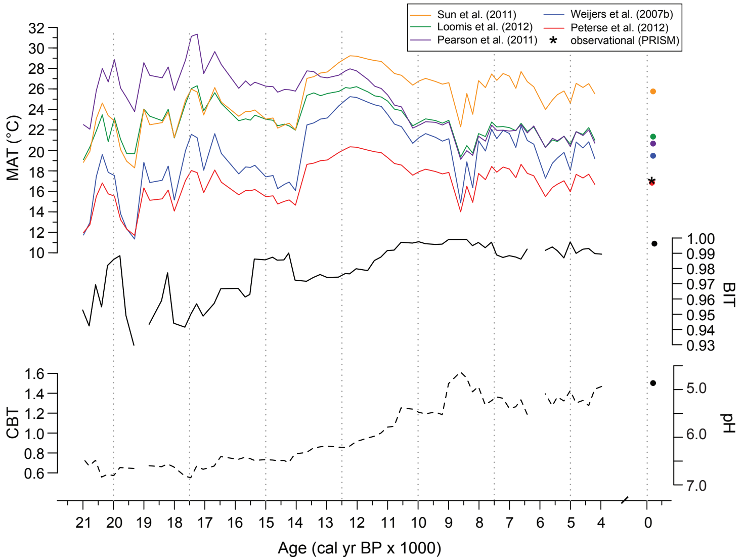
Supplementary Figure 1. brGDGT-based mean annual temperature (MAT) reconstructions at White Pond, SC based on the calibrations of Peterse et al., 2012 (red line), Weijers et al., 2007b (blue), Loomis et al., 2012 (green), Pearson et al., 2011 (purple), and Sun et al., 2011 (orange). MAT reconstructions are plotted against the BIT index (black), and CBT values and inferred pH (dashed line).
