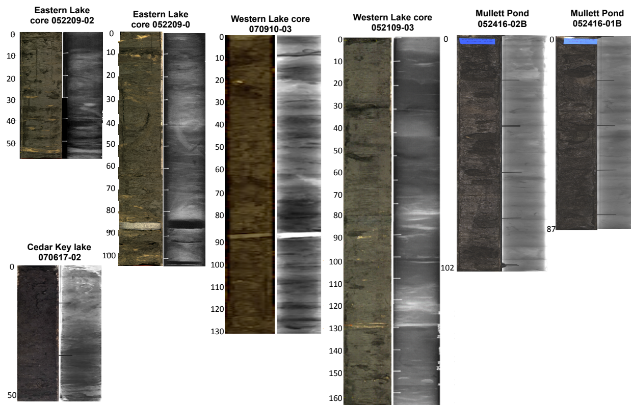
Supplementary Figure 1. Digital images and X-radiographs of sediment cores from coastal lakes in north Florida. The numbers mark the depths in each core in centimeter (cm).
