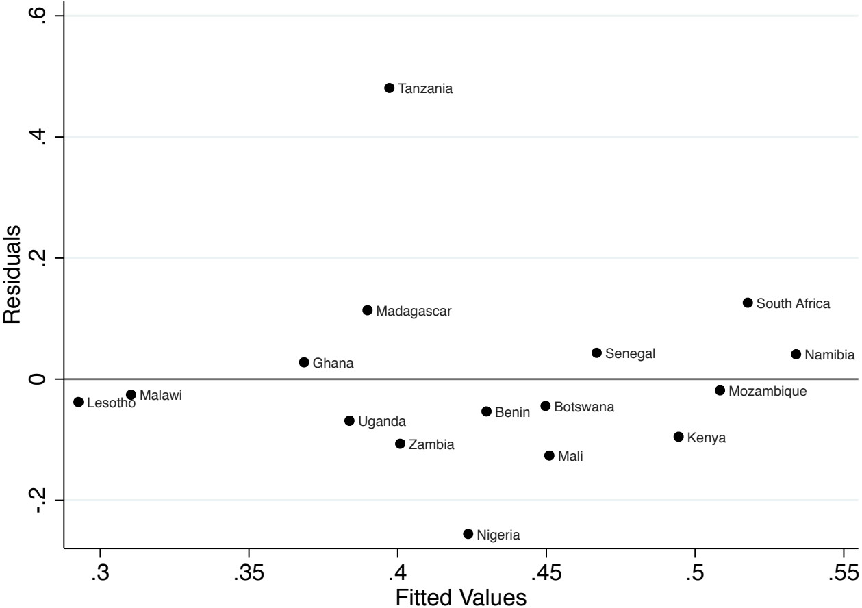
Figure A.1: Residuals vs. Fitted Values for Model 1 of Table A.7
