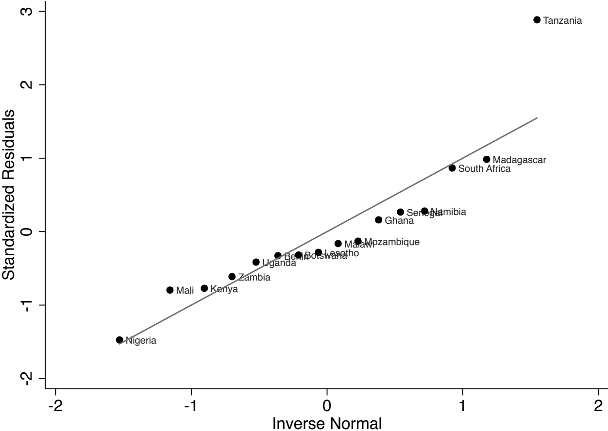
Figure A.2: Standardized Residuals vs. Quintiles of a Normal Distribution for Model 1 of Table A.7
