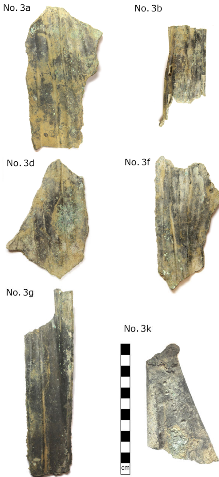
ONLINE FIG. 1. Pieces of drapery from a bronze statue (APPENDIX 3, no. 3). (All photographs by Eve Andreski; rights holder: Bristol City Council; used under CC BY attribution licence)
