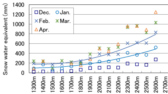
Fig. 9. Relationship between snow water equivalent (averaged over 10 years) and elevation. The regression curves describe data obtained in January and February.
