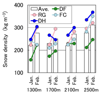
Fig. 11. Relationship between elevation and average snowpack density.
