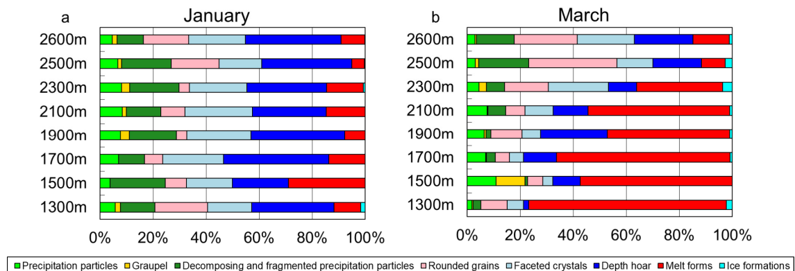
Fig. 5. Distribution ratio of grain shapes in (a) January and (b) March (winter values averaged across 10 years).
