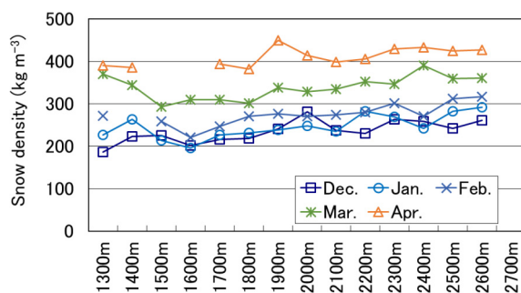
Fig. 8. Relationship between average snowpack density and elevation (values averaged across 10 years).
