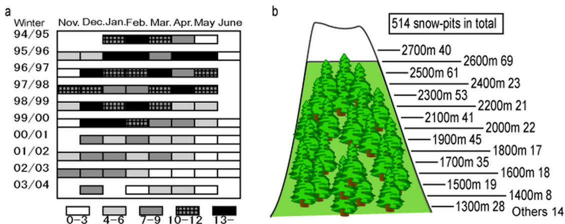
Fig. 3. Number of full snow-pit observations during the decade from 1995 to 2004: (a) in each winter season and month; (b) totals for each study plot.
