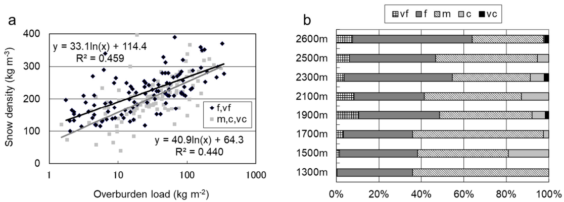
Fig. 7. Grain size of decomposing and fragmented precipitation particles from December to February: (a) relationship with overburden load; (b) frequency of grain size classes.
