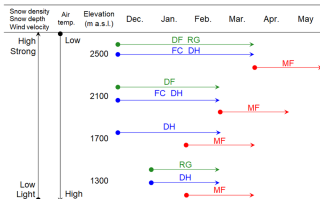
Fig. 12. Temporal transitions of grain shapes at different elevations.
