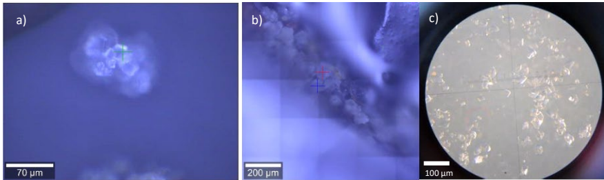
Figure S1. Photographs of carbonate-mineral crystals of a) calcite, b) and dolomite using confocal Raman microscopy. Photos: Gernot Nehrke, and c) ikaite using Leica microscope. Photo: Daiki Nomura.
