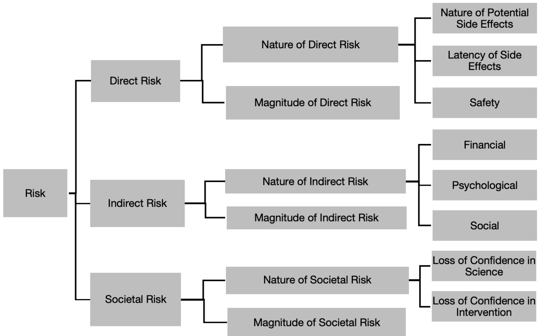
Supplementary Figure 2: Pedigree of factors associated with Risk .
