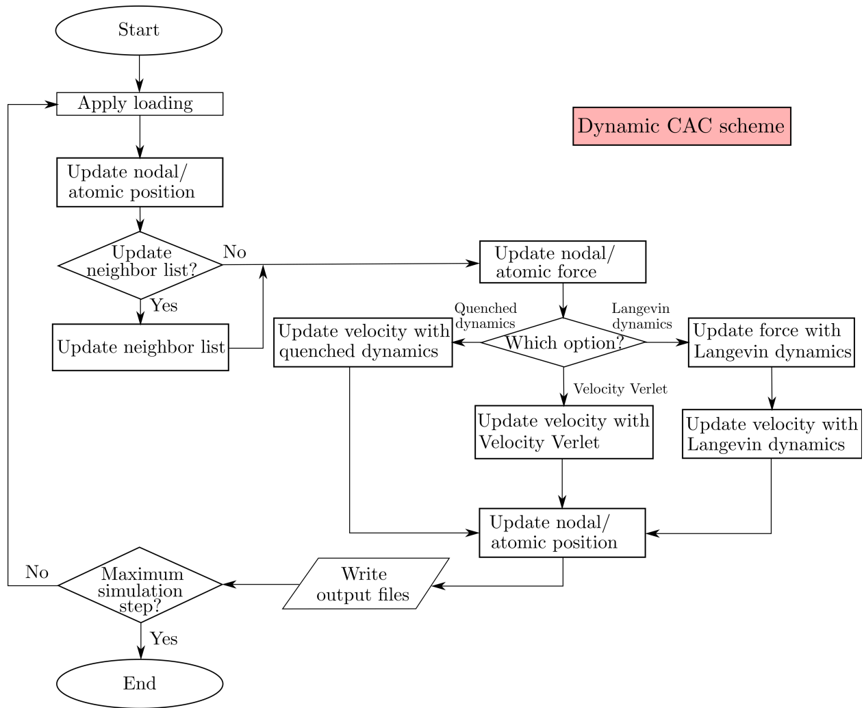
Figure S1: Serial dynamic CAC simulation scheme.
