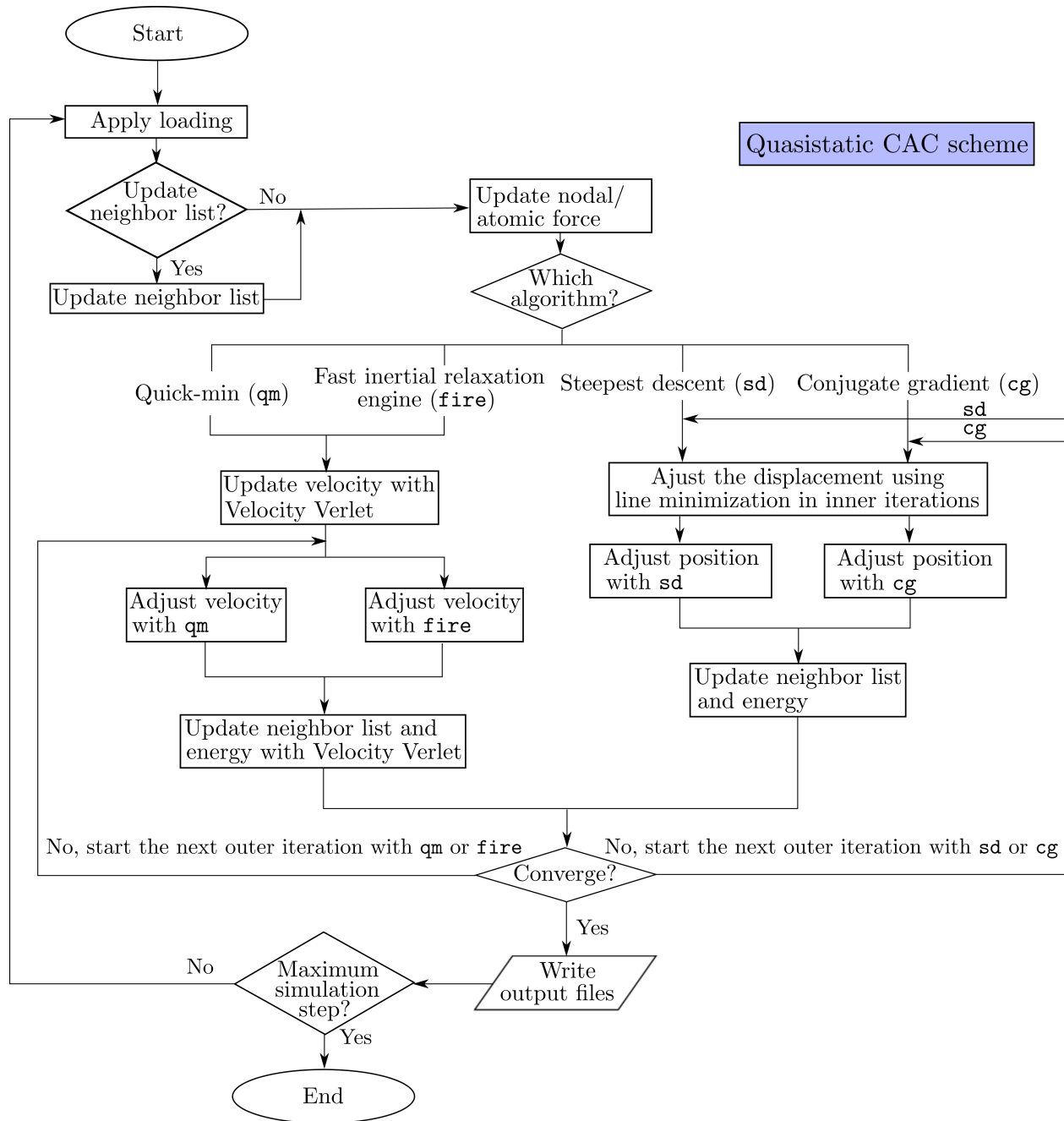
Figure S2: Serial quasistatic CAC simulation scheme.
