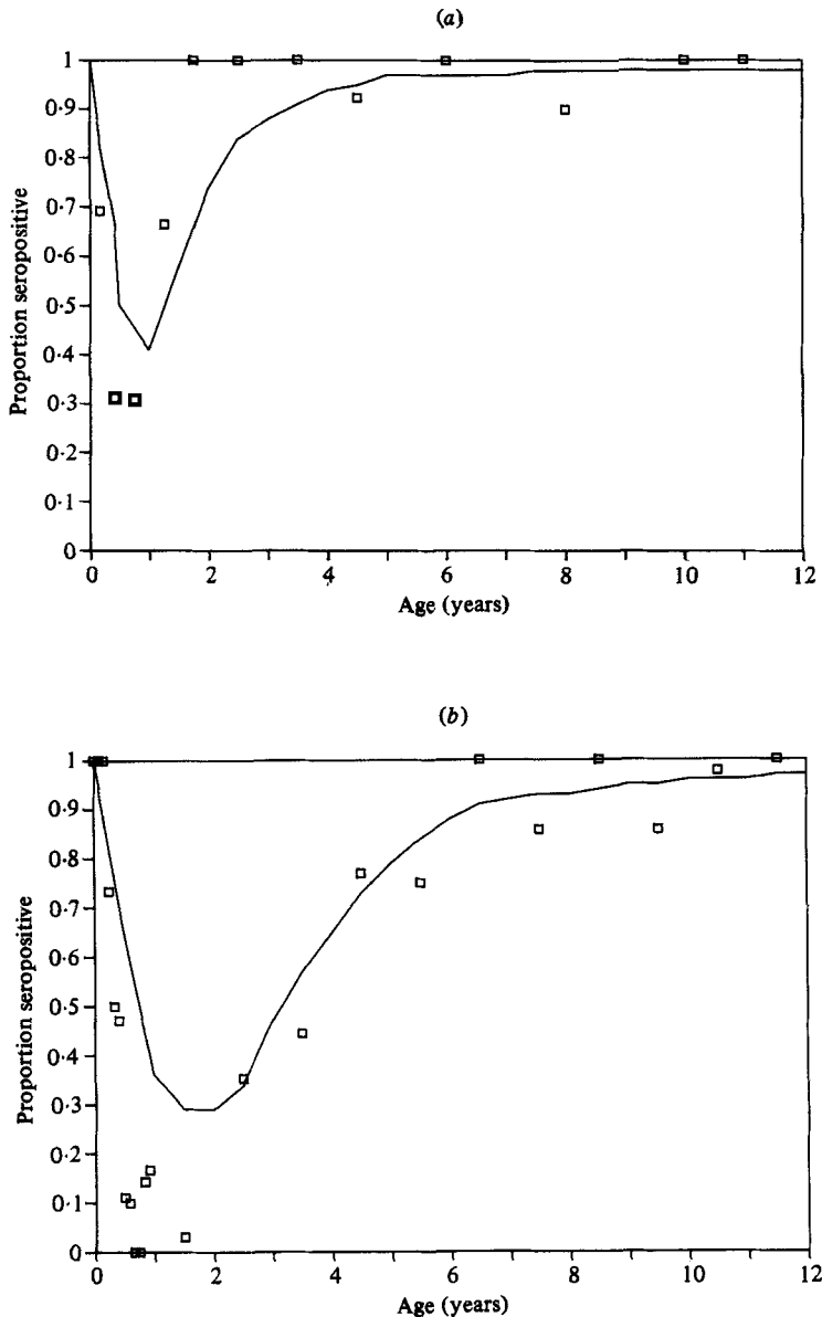
Fig. 1. Serological profiles used in finding optimal ages at vaccination. The figures show raw data ( \square ) and (—) typical serological profiles from model solutions. (a) Serology drawn in Dakar, Senegal in 1957 (Boue, 1964). (b) Serology drawn from Bangkok, Thailand in 1967 (Ueda et al. 1967).
