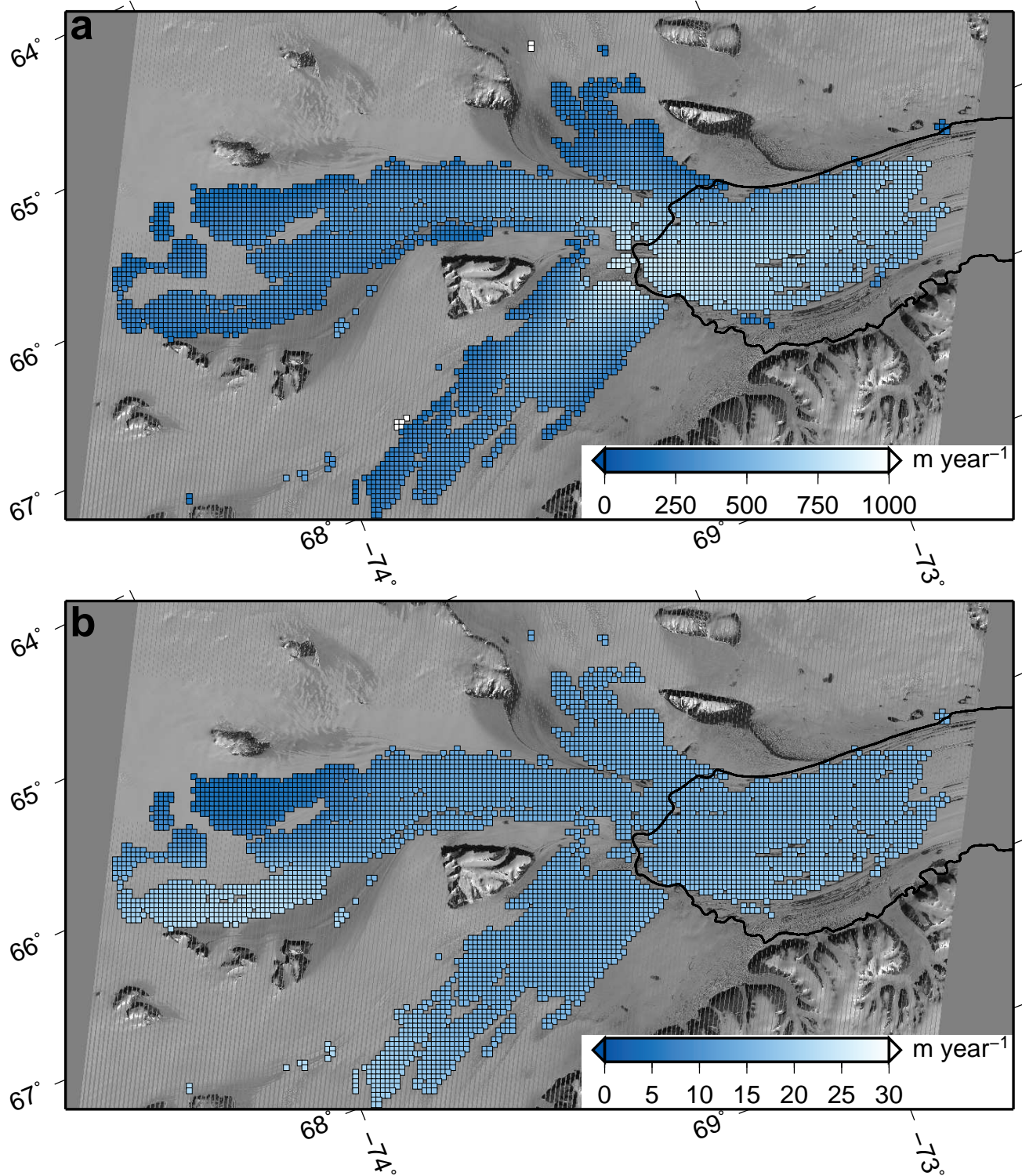
Figure 4: a) The coverage of velocities for the 2007/2008 image pairs b) The coverage of errors for the 2007/2008 image pairs
