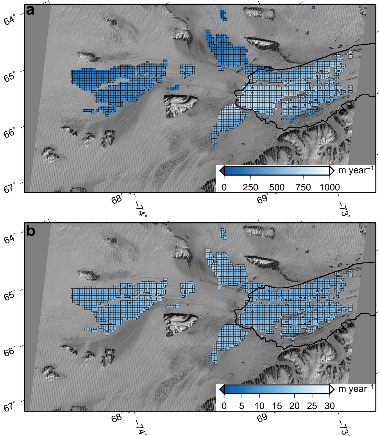
Figure 6: a) The coverage of velocities for the 2010/2011 image pairs b) The coverage of errors for the 2010/2011 image pairs
