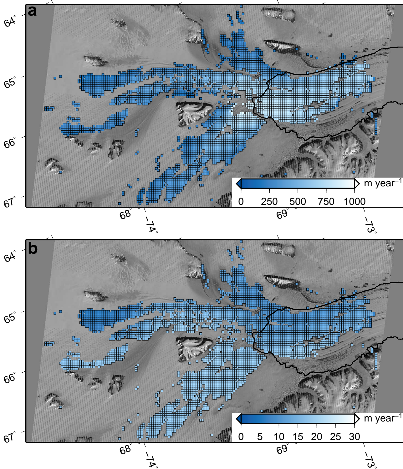
Figure 1: a) The coverage of velocities for the 2004/2005 image pairs b) The coverage of errors for the 2004/2005 image pairs
