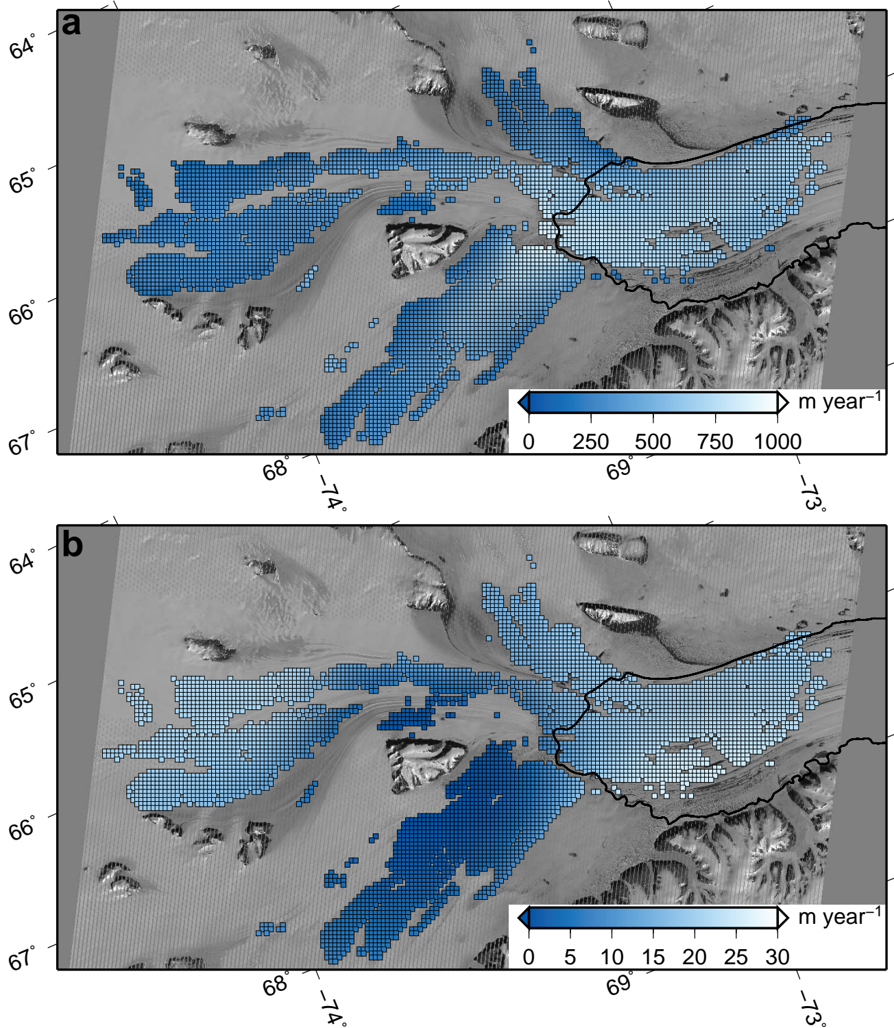
Figure 5: a) The coverage of velocities for the 2008/2009 image pairs b) The coverage of errors for the 2008/2009 image pairs
