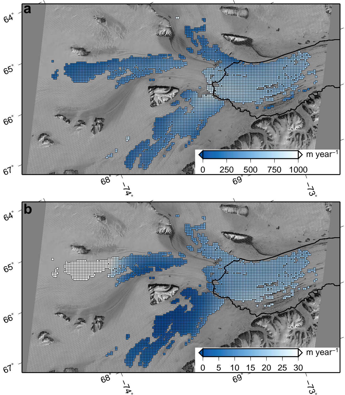
Figure 3: a) The coverage of velocities for the 2006/2007 image pairs b) The coverage of errors for the 2006/2007 image pairs
