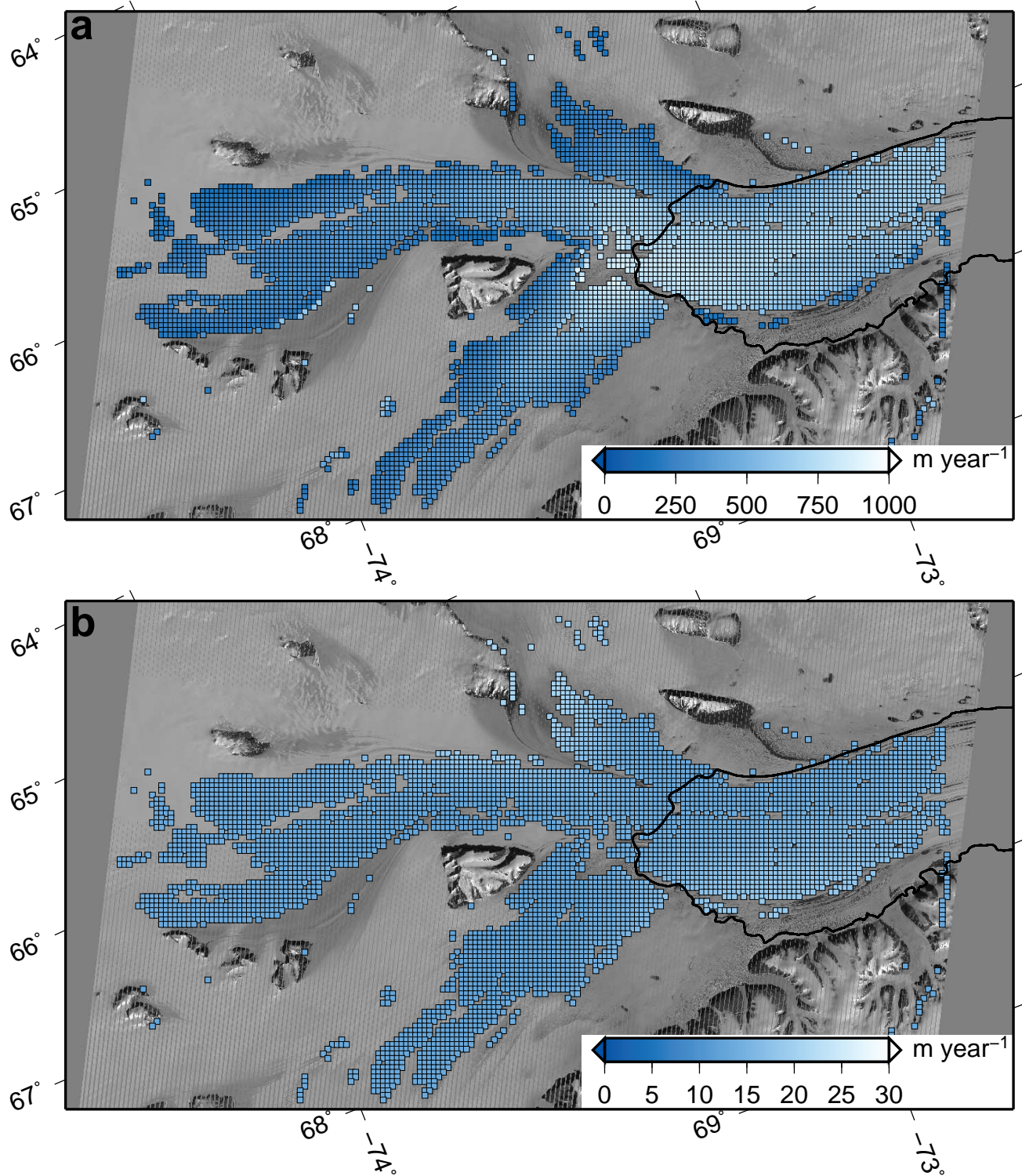
Figure 7: a) The coverage of velocities for the 2011/2012 image pairs b) The coverage of errors for the 2011/2012 image pairs
