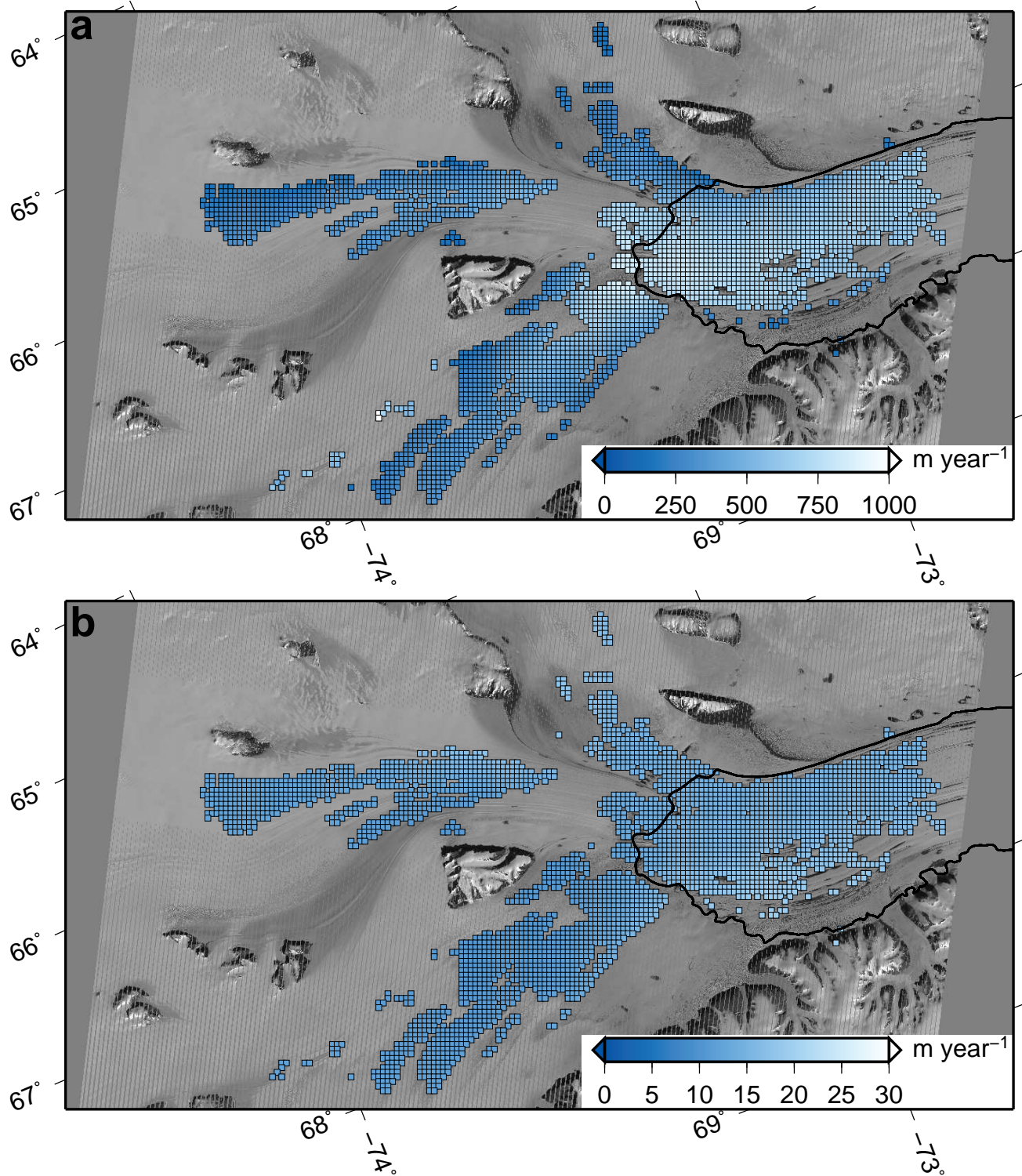
Figure 2: a) The coverage of velocities for the 2005/2006 image pairs b) The coverage of errors for the 2005/2006 image pairs
