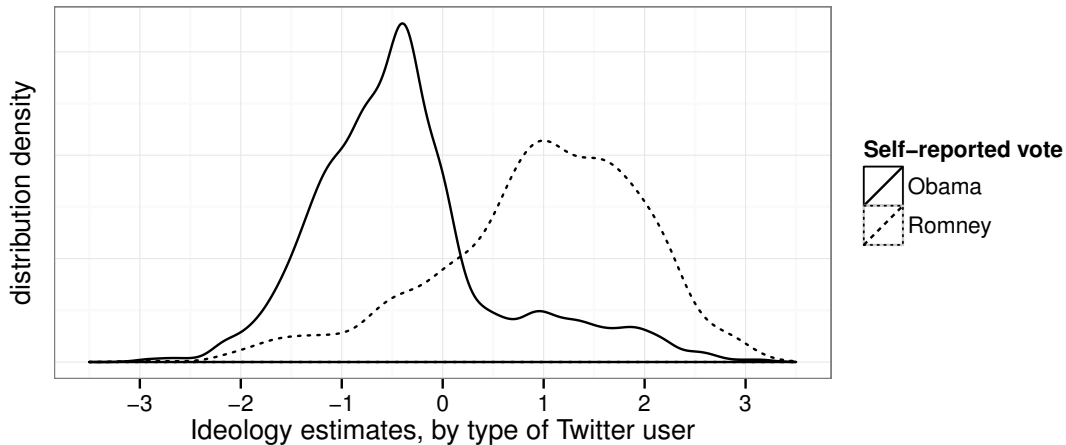
Figure 4: Distribution of Users' Ideal Points, by Self-Reported Votes
