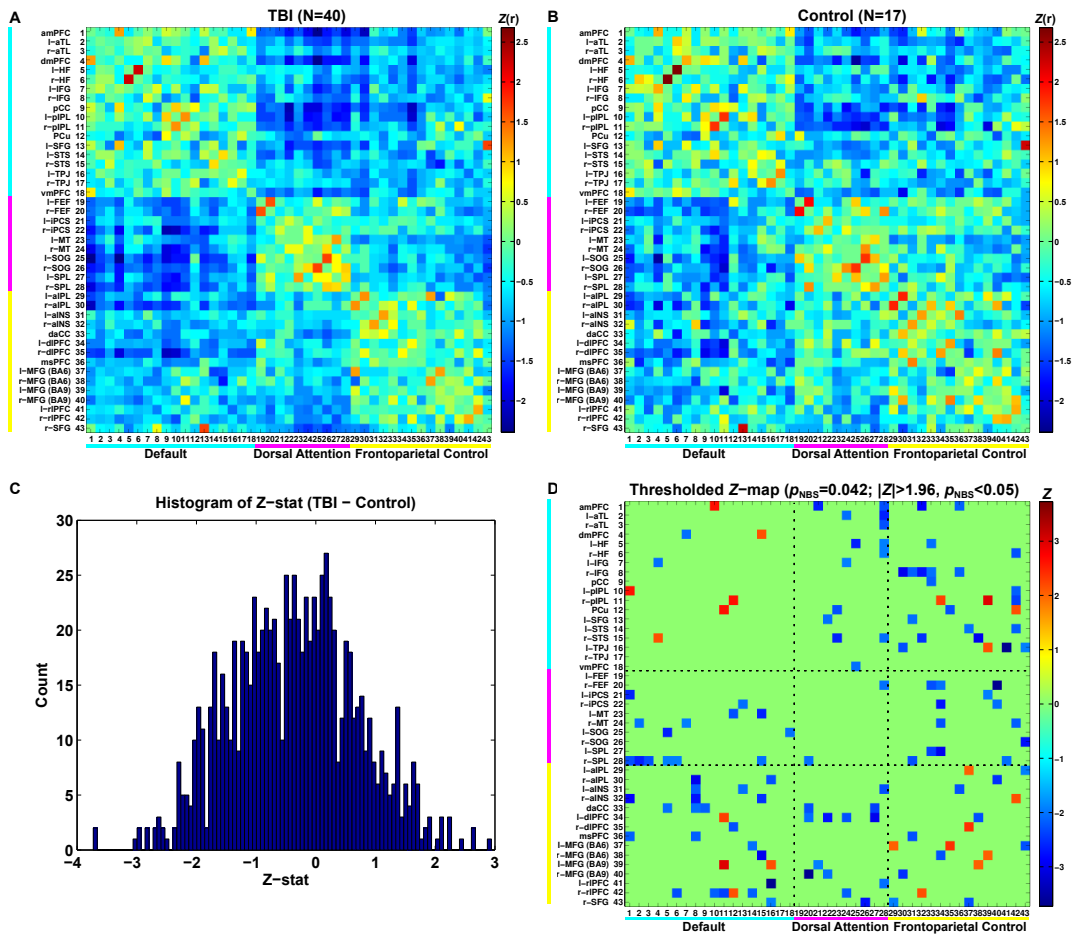
Fig. S10. Group comparisons of average connectivity matrices based on partial correlation coefficients. (A): Average connectivity of the TBI group. (B): Average connectivity of the control group. (C): Histogram for Z-statistics of group comparisons on average connectivity. (D) Thresholded Z-statistic map for group comparisons ( p_{\text{NBS}} < 0.05 at |Z| > 1.96 ). Colorbars in (A) and (B) represent Fisher's Z-transformed correlation coefficients.
