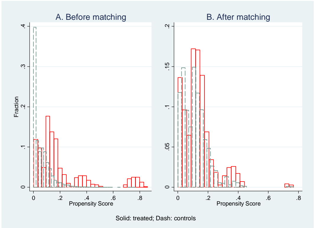
Figure A1. Histogram of estimated propensity matching score ( n=4 cal 0.001) close to national park entrances versus far from parks
