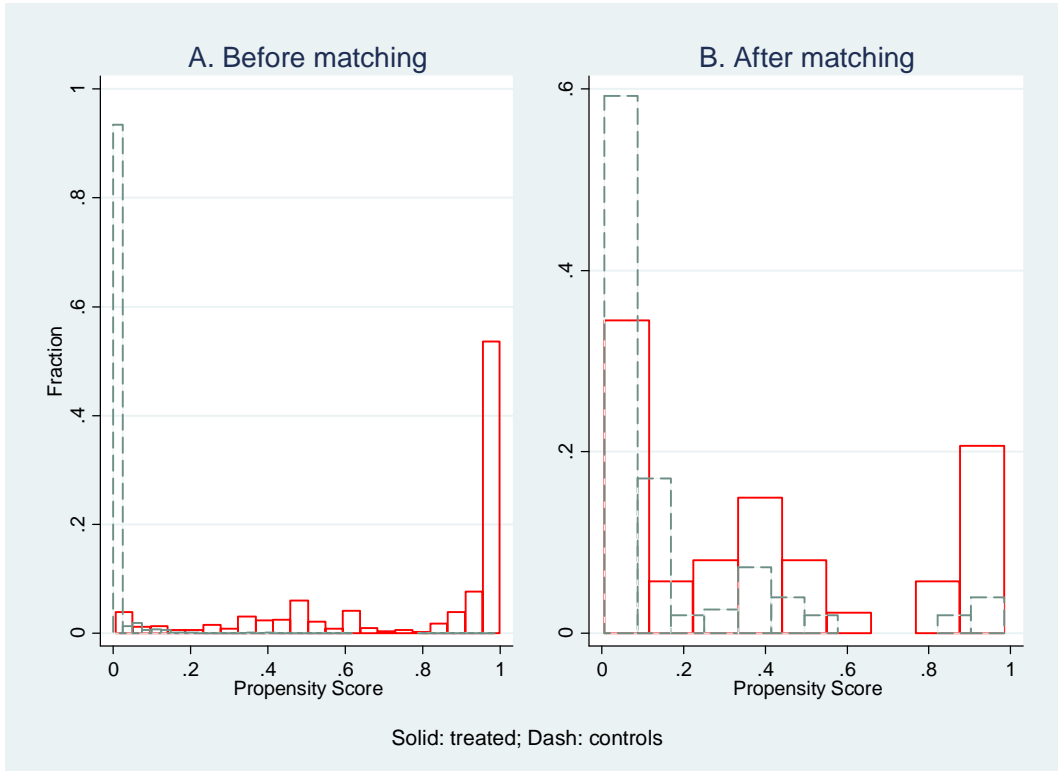
Figure A2. Histogram of estimated propensity matching score ( n=4 cal 0.001) far from national park entrances versus far from parks
