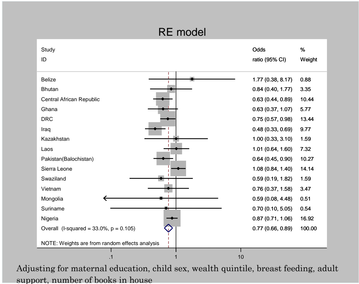
Figure 5: Effect of severe stunting on physical development, ages 36-59 months, MICS4.
