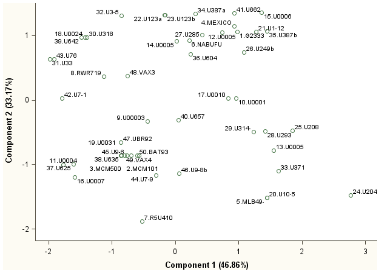
Figure S1. Graphical plot of principal component analysis shows high genetic variations among 50 Mesoamerican germplasm based on growth habits and seed attributes. Germplasm with phenotypic similarity grouped together such as 3- MCM5001, 2-MCM101 in the lower left corner of the plot.
