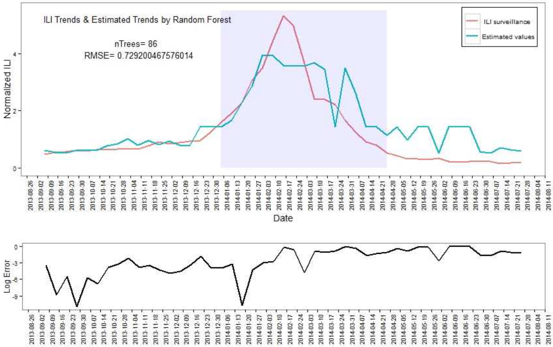
Figure S3. Detection and error based on the Random Forest model.
