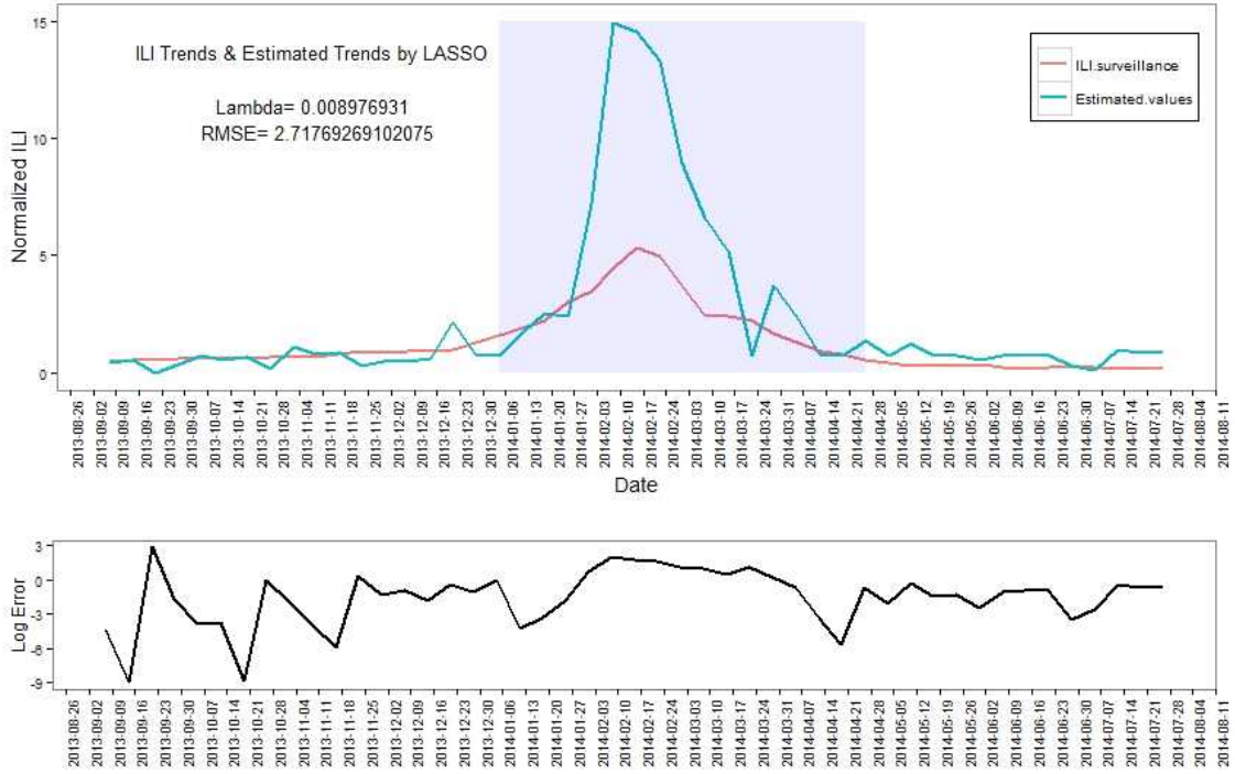
Figure S2. Detection and error based on the lasso model.
