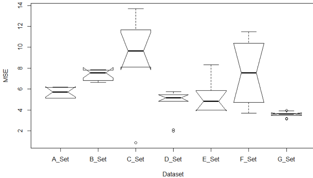
Figure S1. Identification of the optimal dataset by 10 times experiments of Lasso. ‘B set (Blog set)’ means a dataset including keywords and its volumes generated from web blog posts. ‘C set (Twitter set)’ means a dataset including keywords and its volumes generated from twitter. ‘A set’ has been constructed as average of keyword volumes generated from web blog posts and twitter, respectively. ‘D, E, F and G set’ are merged dataset based on A, B and C set.
