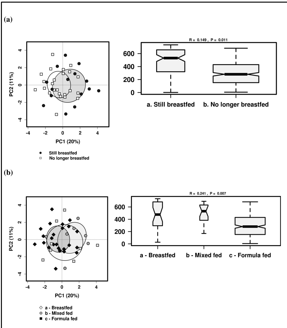
Supplementary Figure 3: Investigation of different factors on the gut microbiota diversity in one year old children who have been exposed to all possible antibiotics (n=39) using PCA and Anosim (Bray-Curtis) at genus level (a) breastfeeding status (b) feeding patterns.
