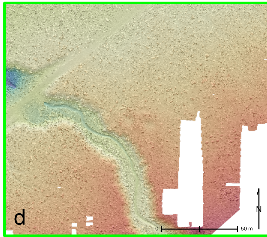
Agisoft PhotoScan
