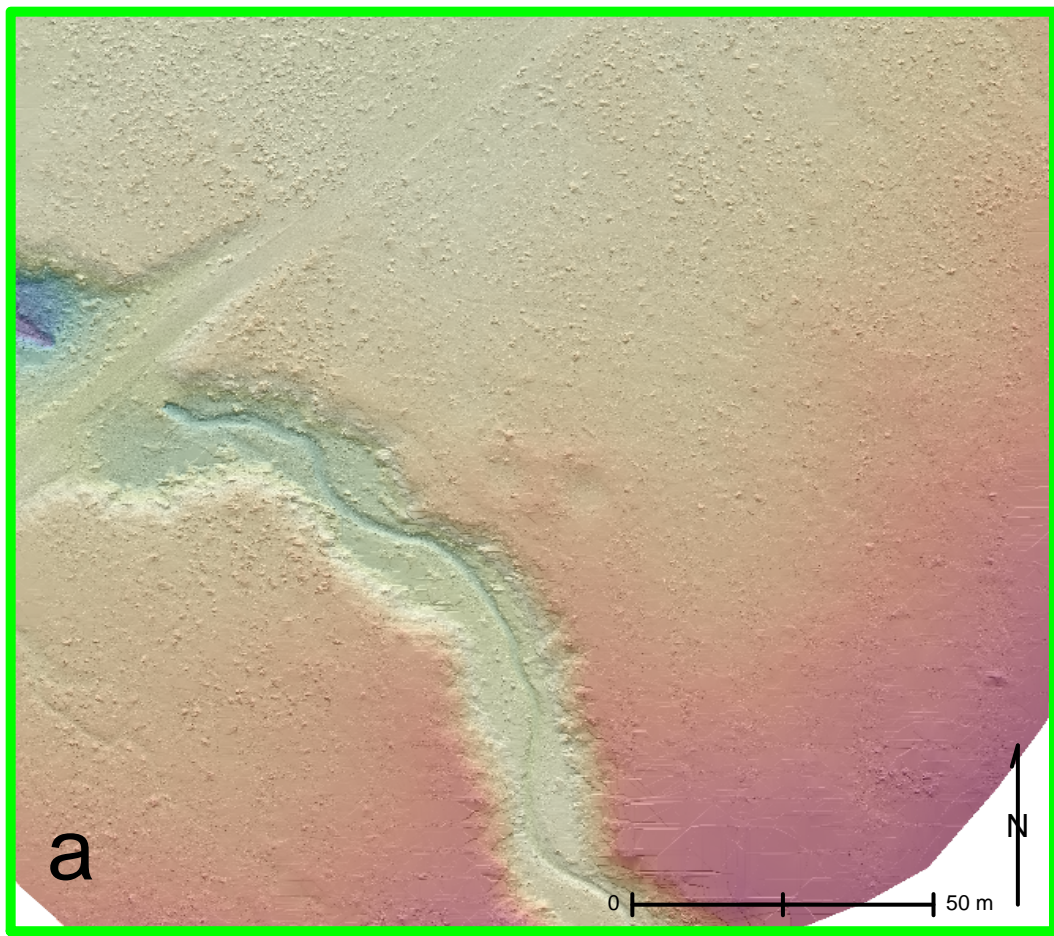
OpenDroneMap
